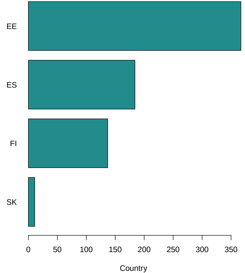
Reduced Sample
