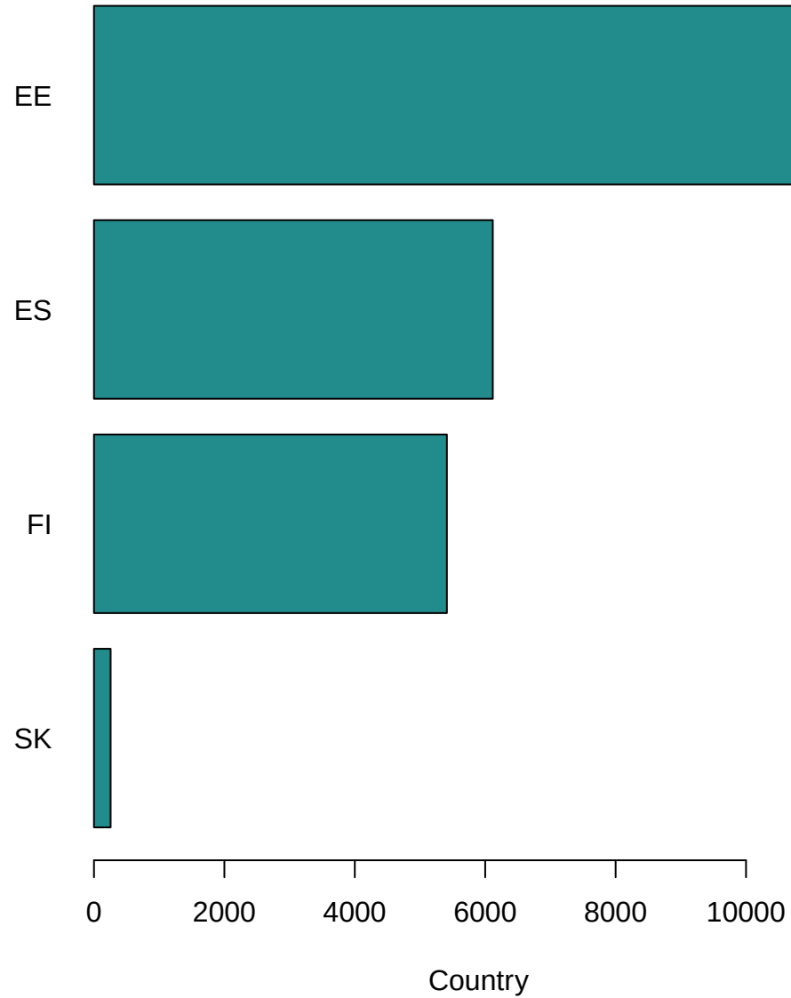
Initial Sample
