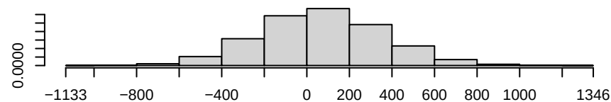
Density of b1cov.b1_age
