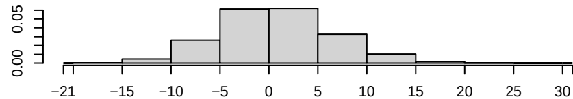
Density of b1factor.b1_gender.male
