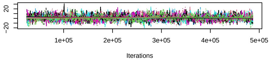
Trace of b1factor.b1_gender.male
