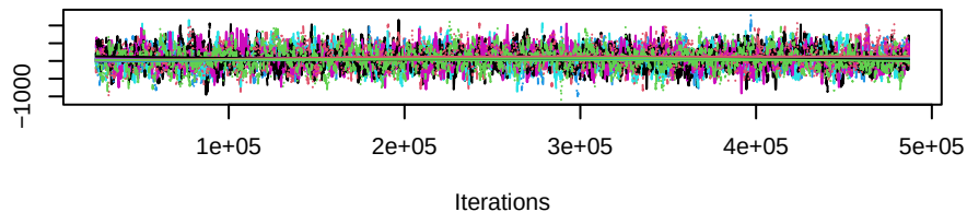
Trace of b1cov.b1_age
