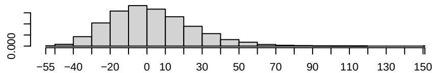
Density of cycle4
