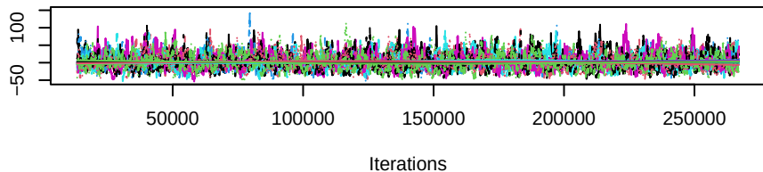
Trace of cycle4
