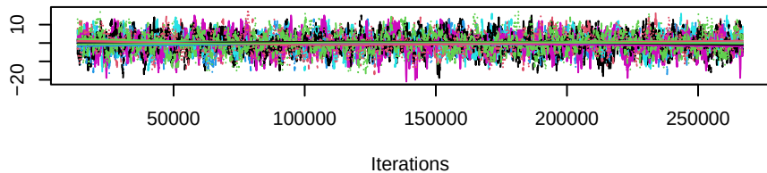
Trace of b1degree1
