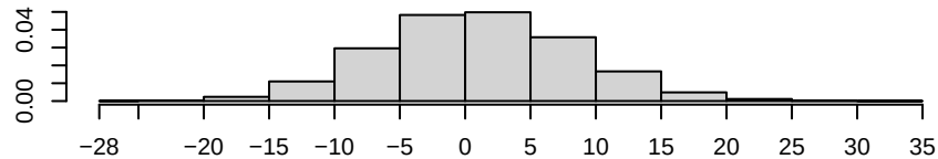
Density of edges
