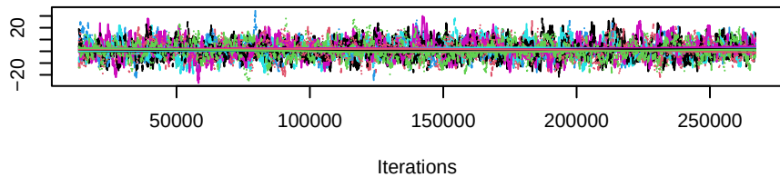
Trace of edges
