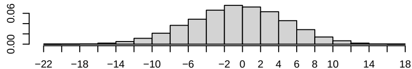
Density of b1degree1
