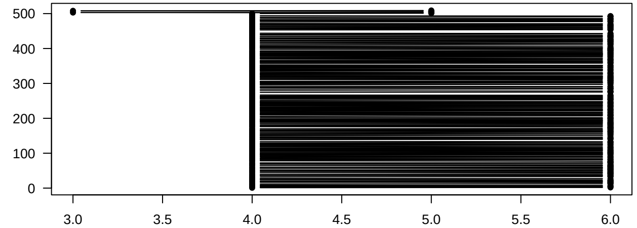
eccentricity
