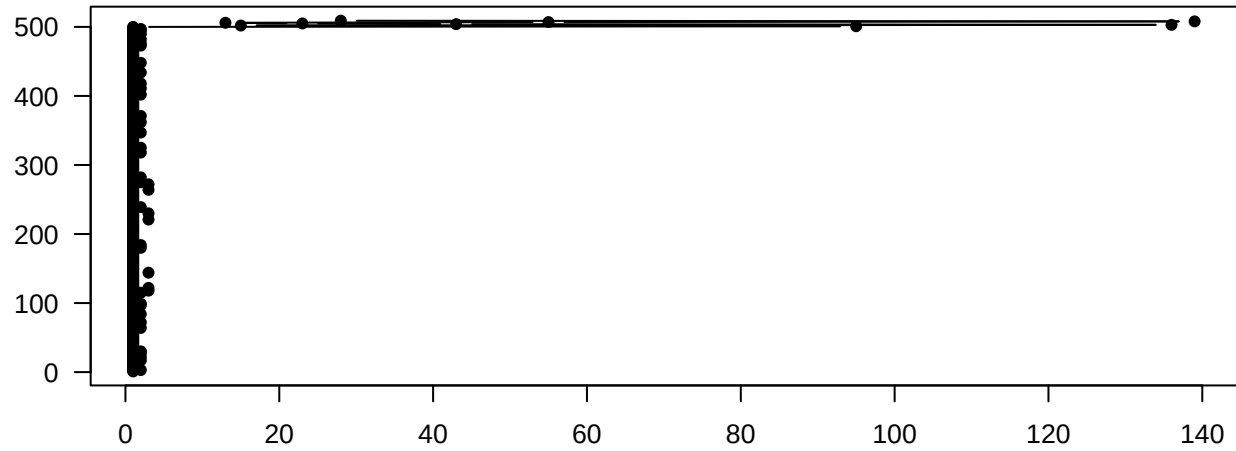
degree
