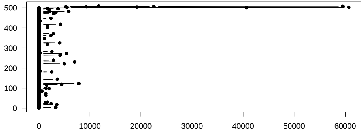
betweenness
