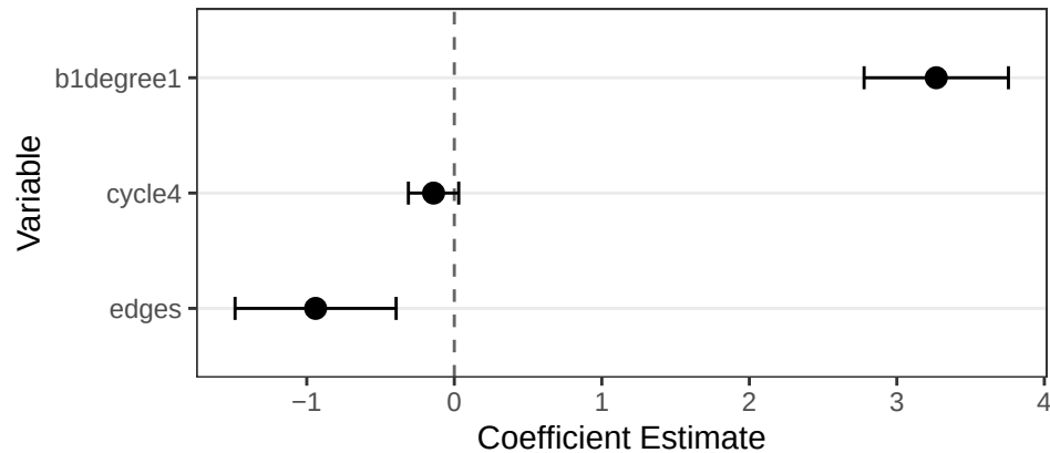
Complete Model
