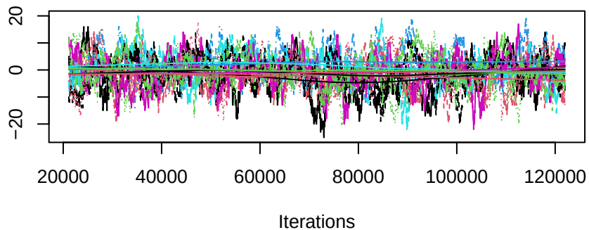
Trace of b1degree1
