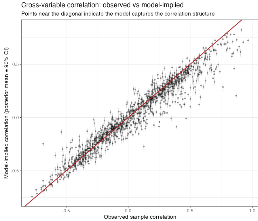
Figure 14: PPC: observed vs predicted feature-pair correlations (K=2 Normal model, P=48 rebuilt data). High correlation ( r \approx 0.98 ) confirms the model captures cross-feature covariance structure. PPC for stage 28 K=3 t-model pending stage 19 rerun.
