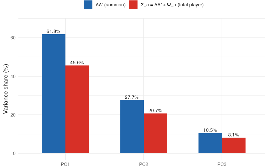
Figure 3: Variance shares per PC for \hat{\Lambda}\hat{\Lambda}^\top (common factor variance) vs \hat{\Sigma}_a = \hat{\Lambda}\hat{\Lambda}^\top + \hat{\Psi}_a (total player variance). The gap is the per-feature uniqueness \hat{\Psi}_a not explained by the K = 3 shared factors.
