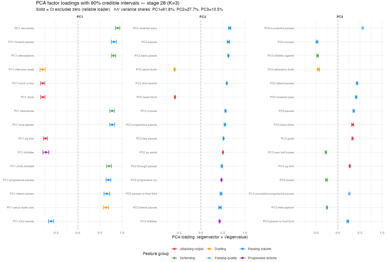
Figure 4: PCA factor loadings (eigenvector \times \sqrt{\text{eigenvalue}} ) with 90% credible intervals (K=3, stage 28, P = 48 ). Solid = CI excludes zero (reliable loader). Positive PC1 = defensive work-rate; negative PC1 = attacking output.
