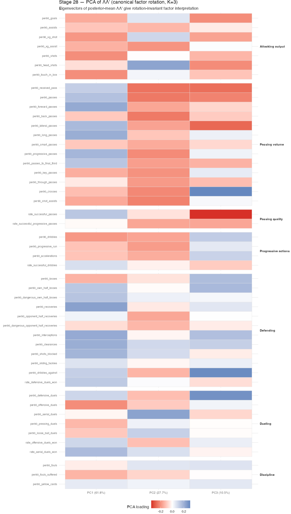
Figure 3: PCA-rotated loadings: eigenvectors of posterior-mean \hat{\Lambda}\hat{\Lambda}^\top (K=3, stage 28).
