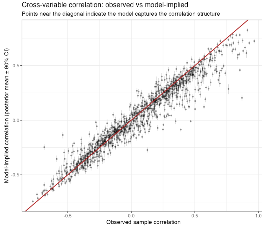
Figure 12: PPC: observed vs predicted feature-pair correlations (K=2 Normal model, P=48 rebuilt data). High correlation ( r \approx 0.98 ) confirms the model captures cross-feature covariance structure. PPC for stage 28 K=3 t-model pending stage 19 rerun.
