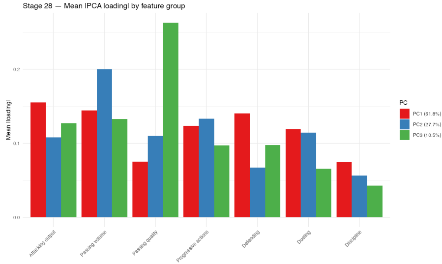
Figure 4: Mean absolute PCA loading by feature group and PC (stage 28, K=3).
