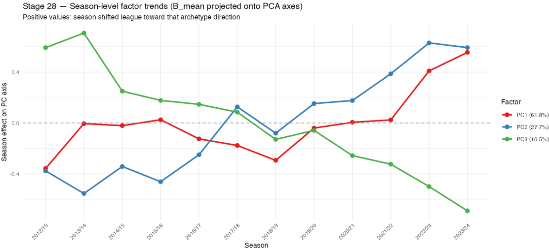
Figure 9: Season-level factor trends: \hat{b}_j projected onto PC1–PC3 axes (2012/13–2023/24). Positive = season shifted the league toward that archetype direction.
