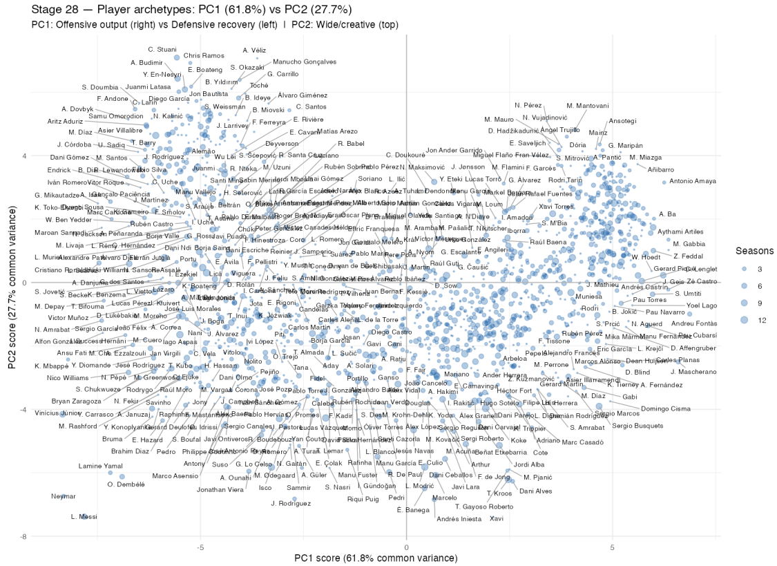
Figure 5: Player archetypes: PC1 vs PC2 score for all 1,529 outfield players. Point size = number of seasons observed. Extreme players labelled.
