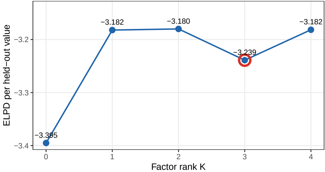
Figure 1: Pathfinder ELPD per held-out value for K = 0, \dots, 4 (rebuilt data, N = 4,586 , P = 48 ).
