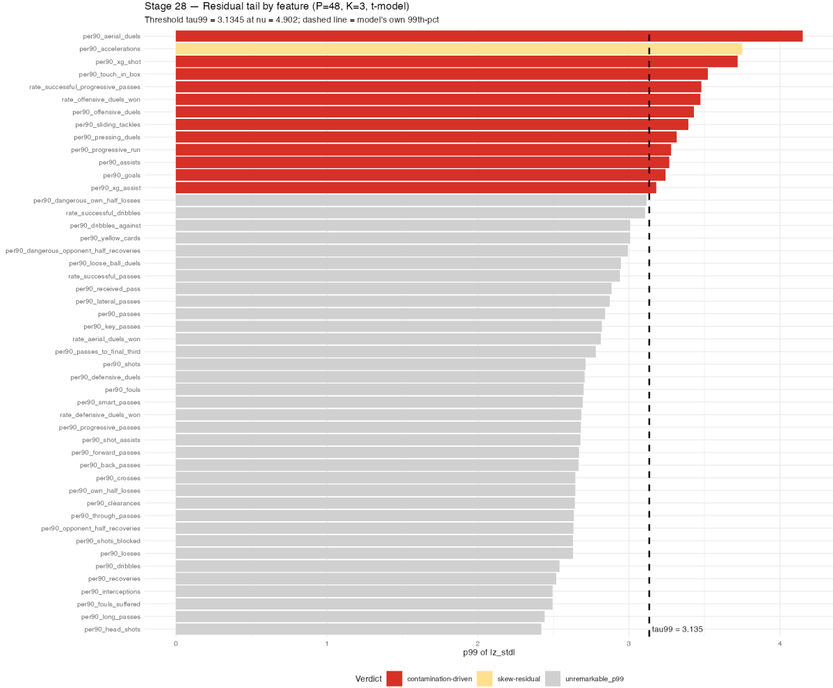
Figure 10: p99 of |z_{np}| for each of the 48 features, coloured by verdict. Dashed line = \tau_{99} = 3.135 (model's own 99th-pct threshold at \hat{\nu} = 4.902 ). Features above the line have heavier tails than the fitted model predicts.
