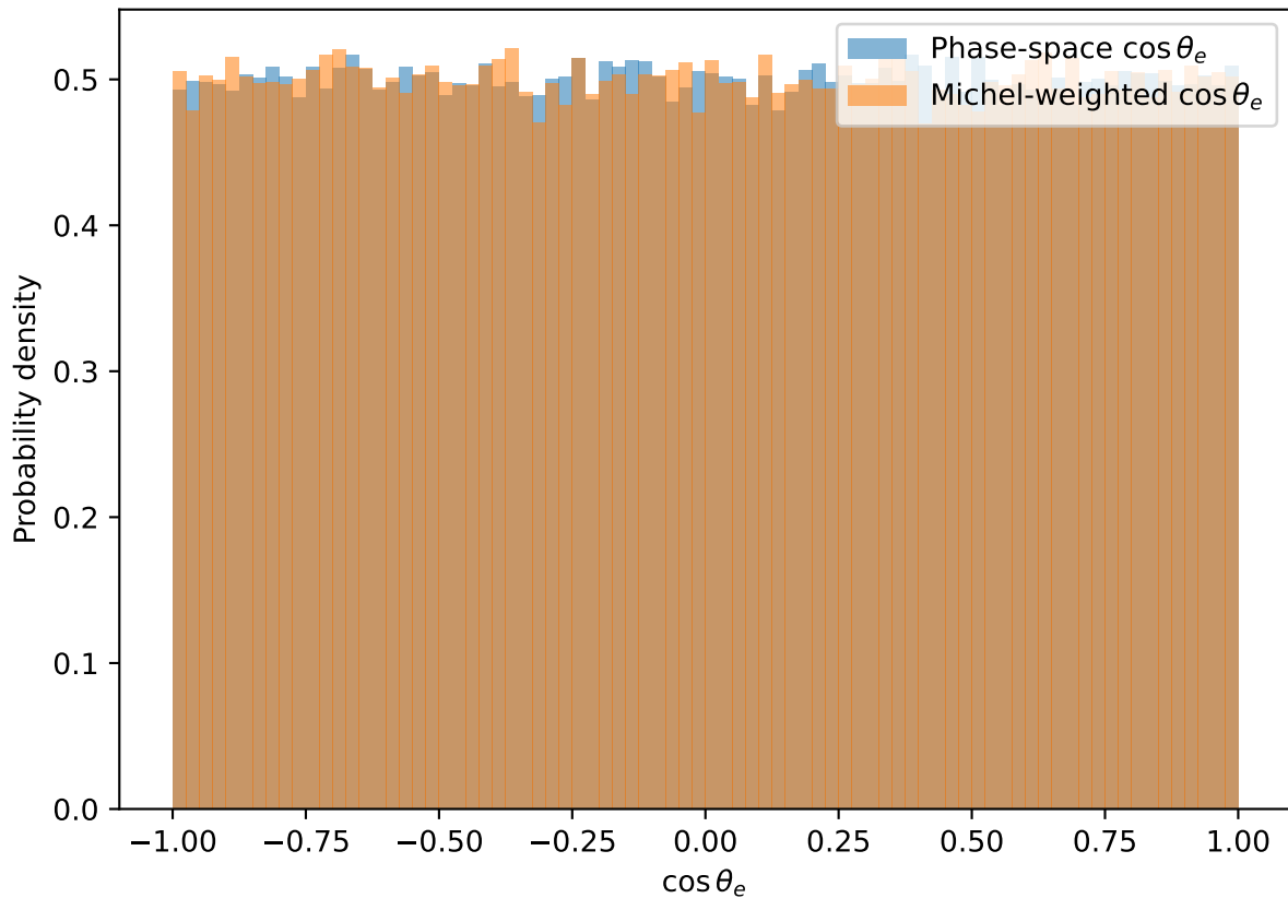
Muon decay: electron direction isotropy check
