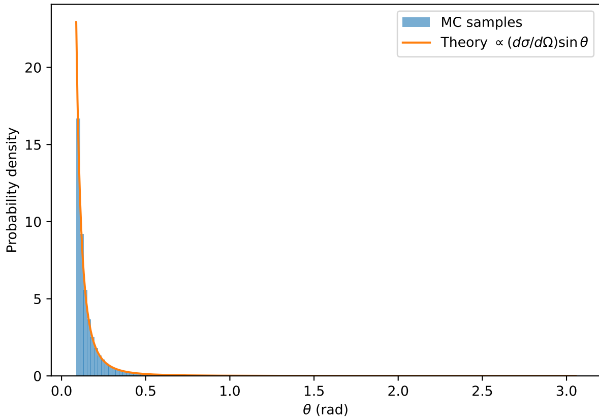
Rutherford \theta sampling validation (importance sampling)
