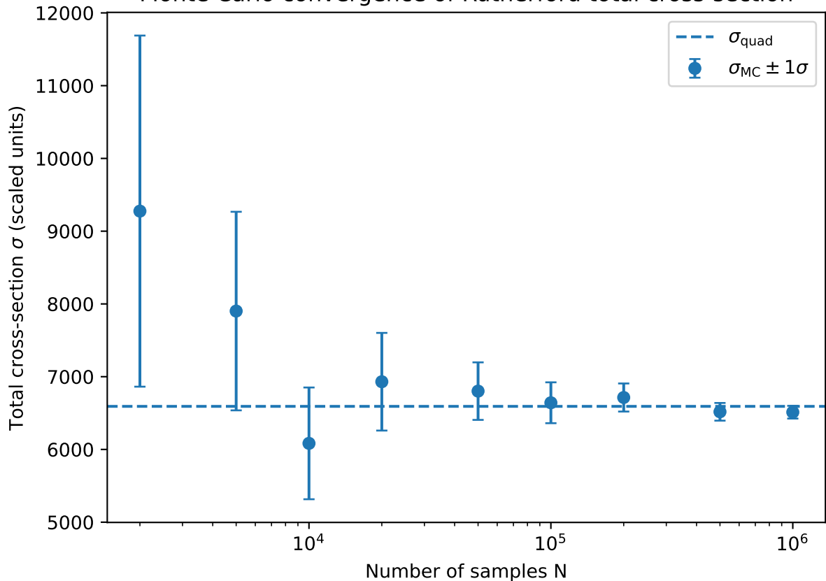
Monte Carlo convergence of Rutherford total cross-section
