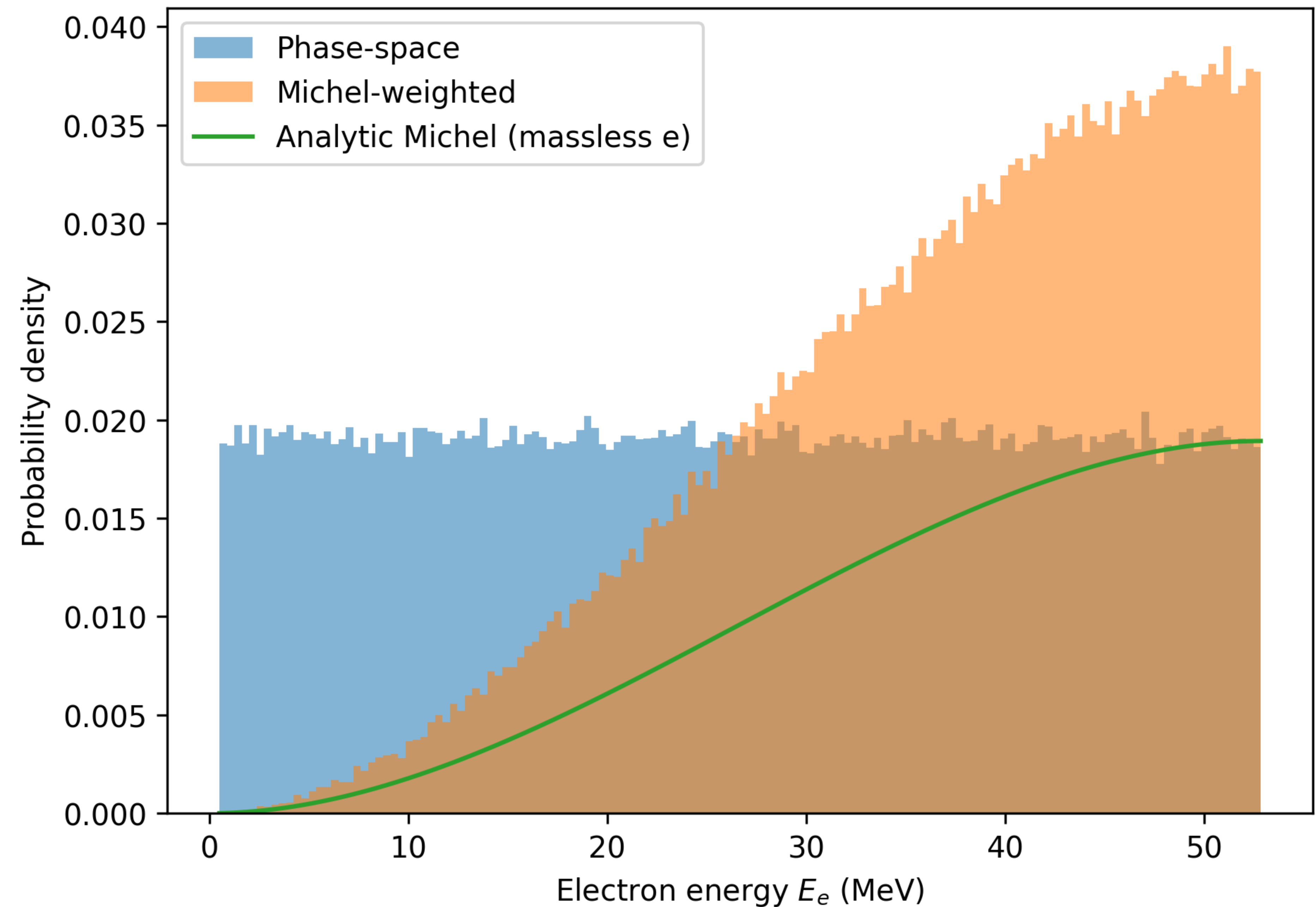
Muon decay: phase-space vs Michel-weighted electron spectrum
