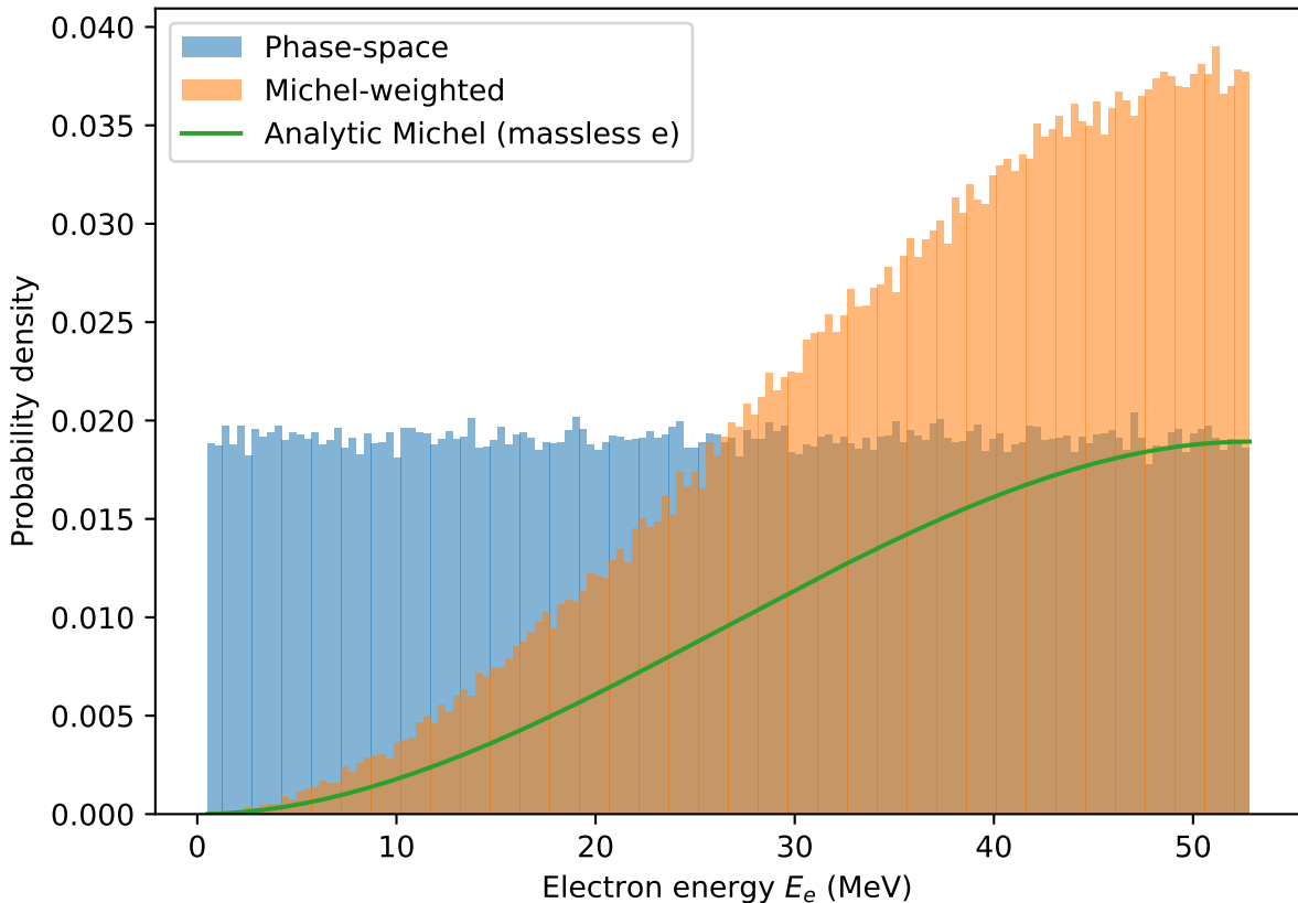
Muon decay: phase-space vs Michel-weighted electron spectrum
