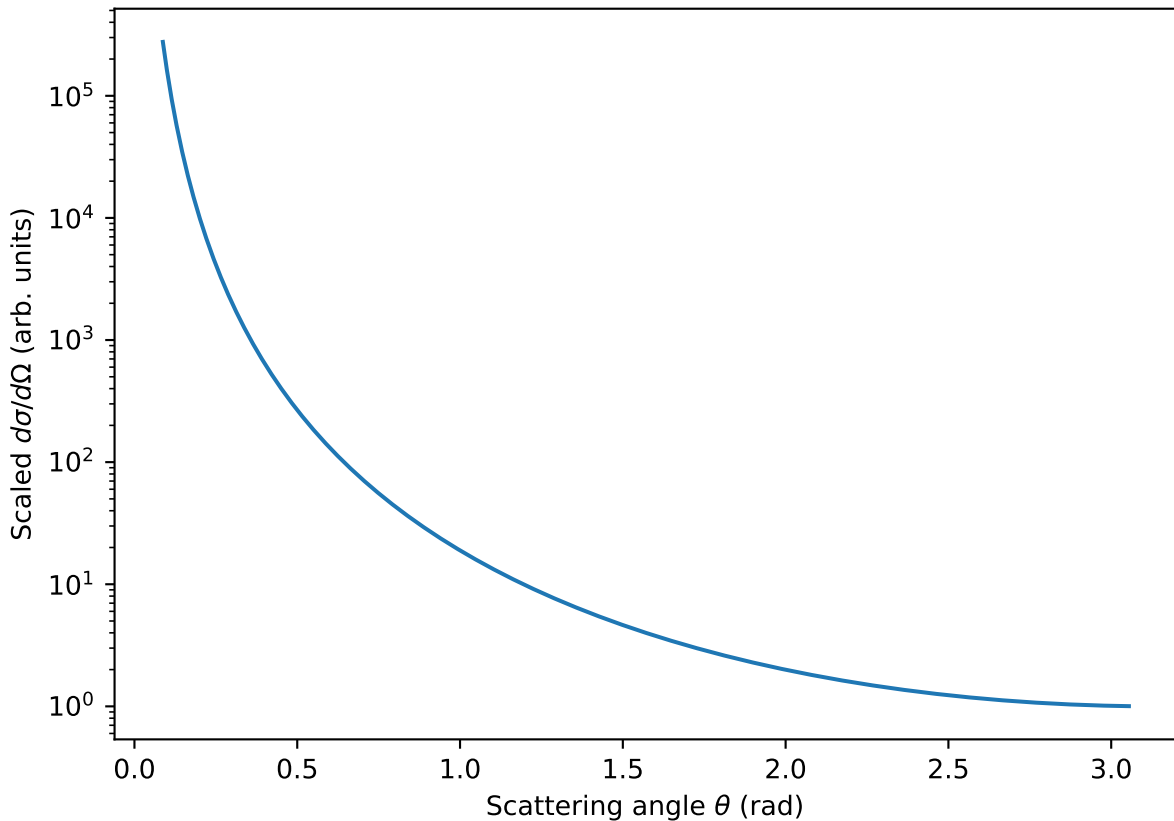
Rutherford angular dependence (with acceptance cuts)
