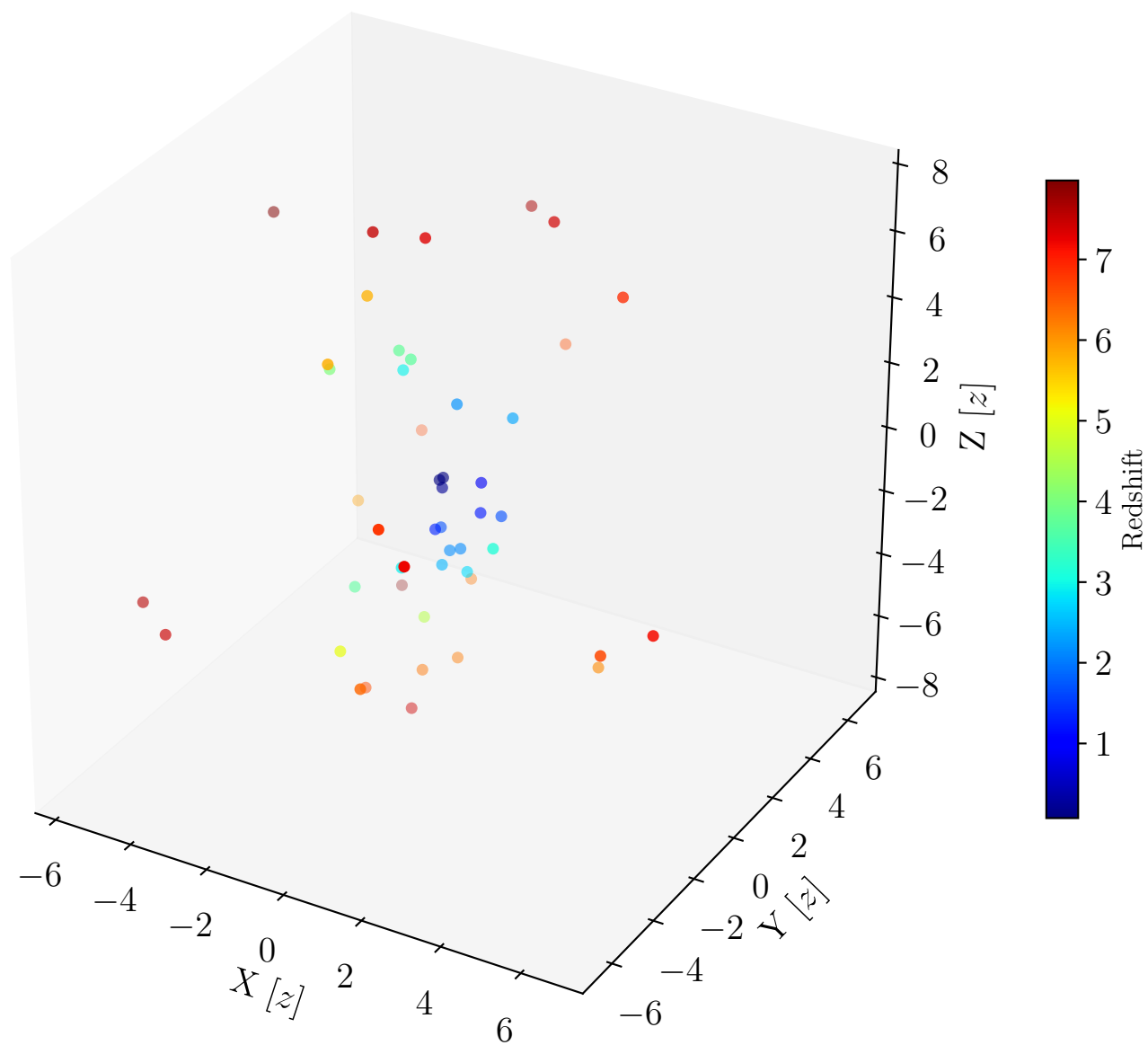
3D Galaxy Distribution (Concentric Shells)
