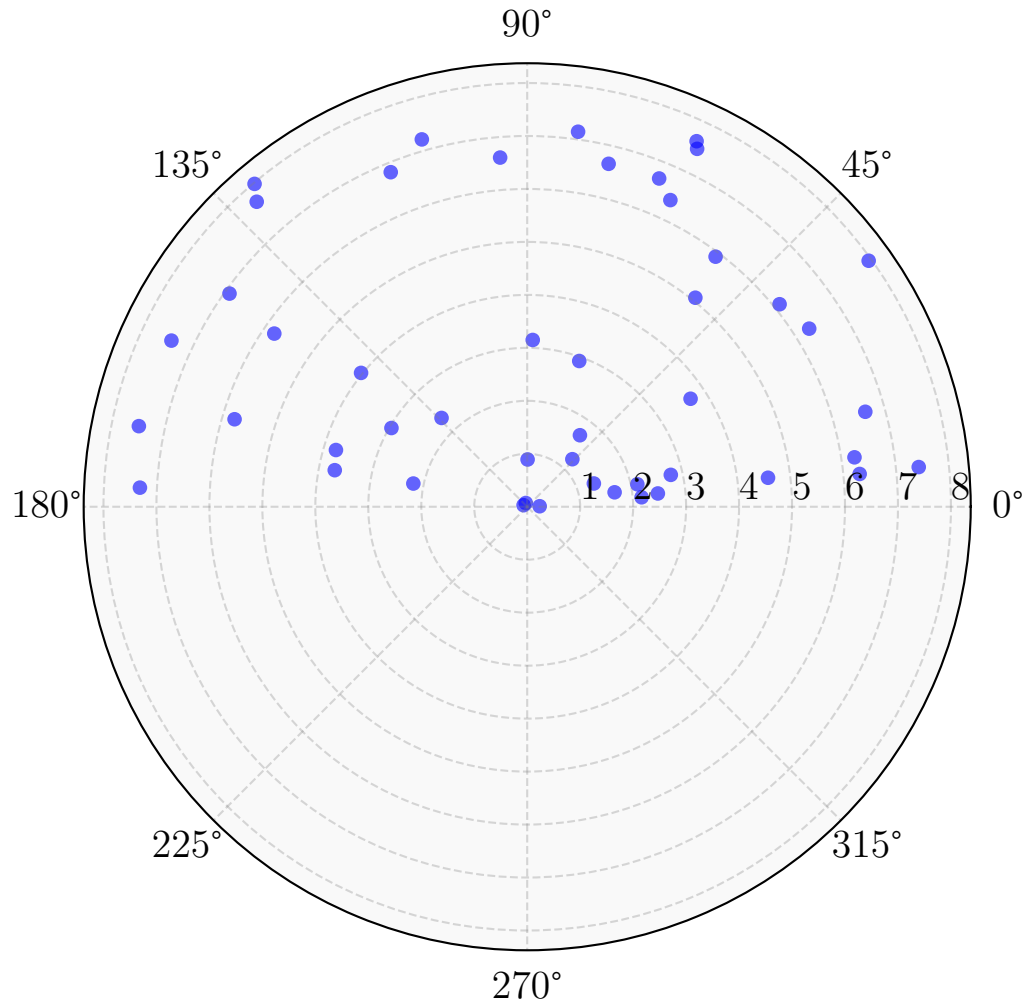
Galaxy Distribution: Dec vs Redshift
