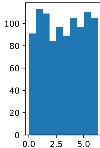
coa_phase
