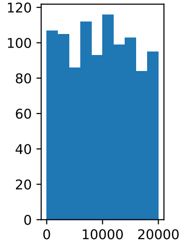
distance
