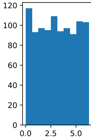
polarization
