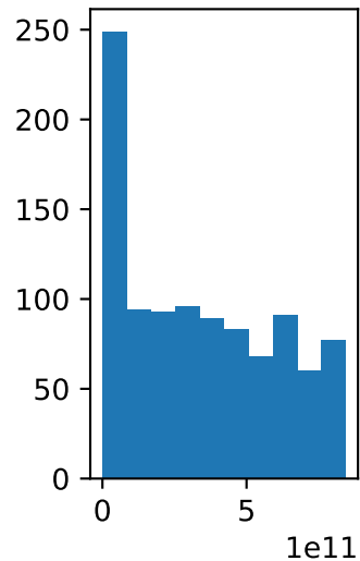
dec
