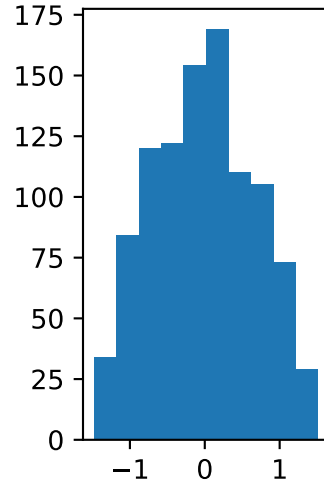
dec
