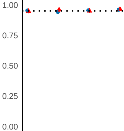
CI Coverage
