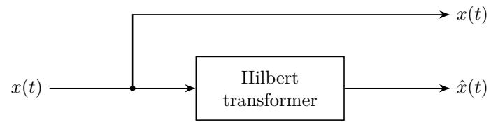
Figure 1: Generation of an analytic signal using a Hilbert transformer.
