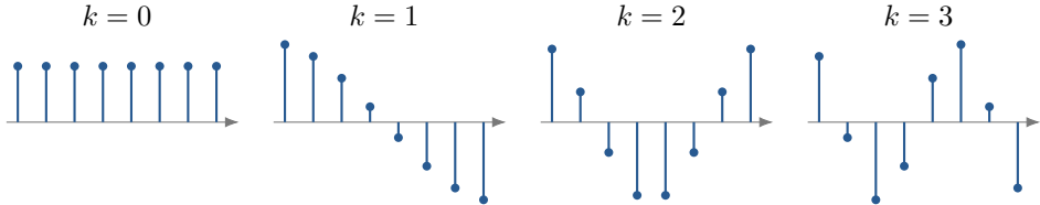
First four DCT-II basis vectors \cos(\frac{\pi(2n+1)k}{2N}) for N = 8 (scaled by w[k]\sqrt{N/2} ), n = 0, \dots, 7 .
