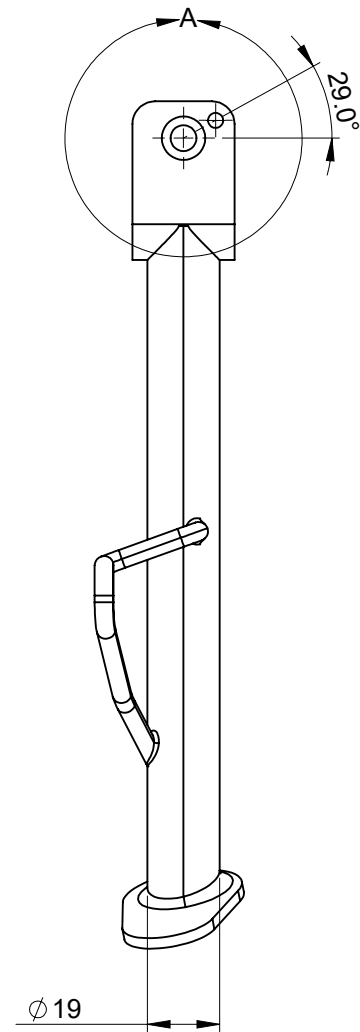
LOCATING PIN HOLE PLACEMENT ON STAND
