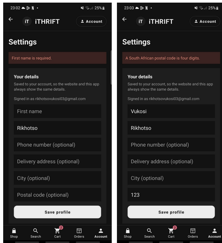
Figure 30: Manual checks on the phone: a blank first name in case 10 (left) and a three-digit postal code in case 11 (right)
