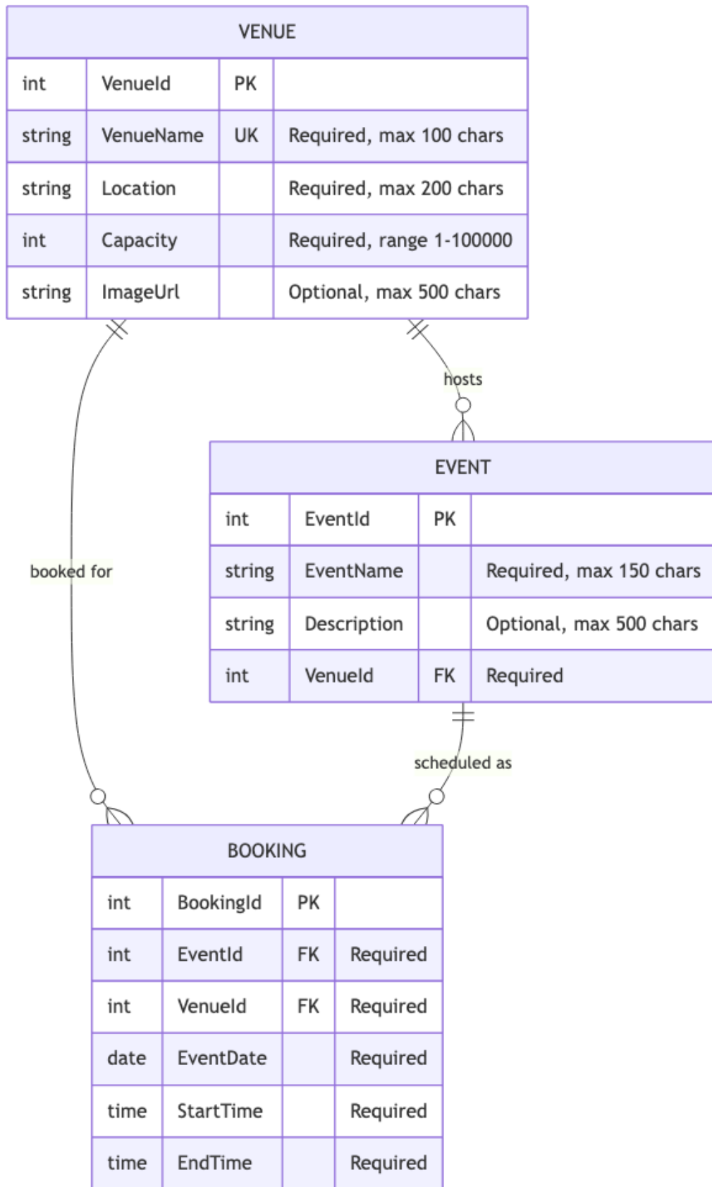
Figure 1: ERD Diagram
