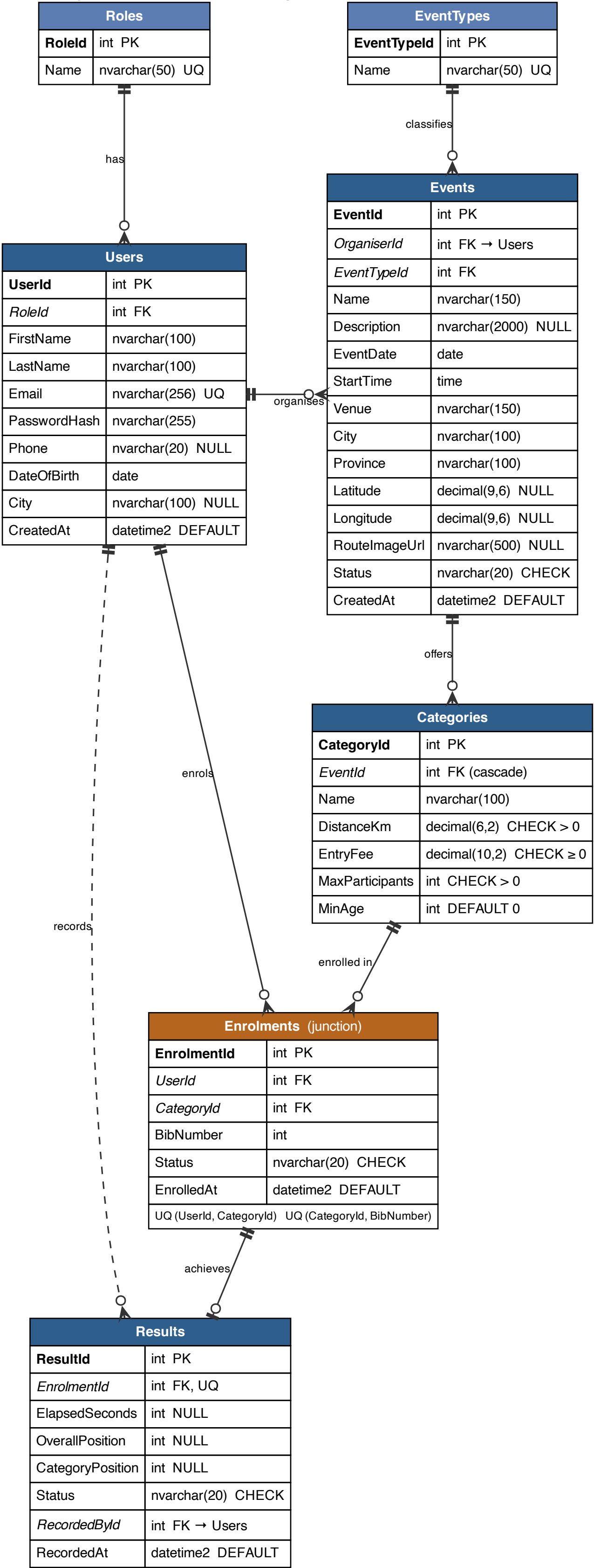
RaceDay - Entity Relationship Diagram (crow's foot) Users M:M Categories is resolved through Enrolments; Enrolments 1 : 0..1 Results
