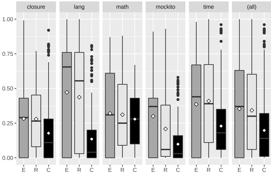
mutation score
