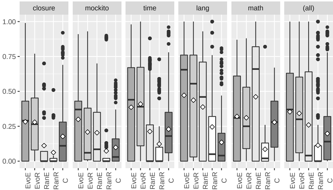
Mutation score
