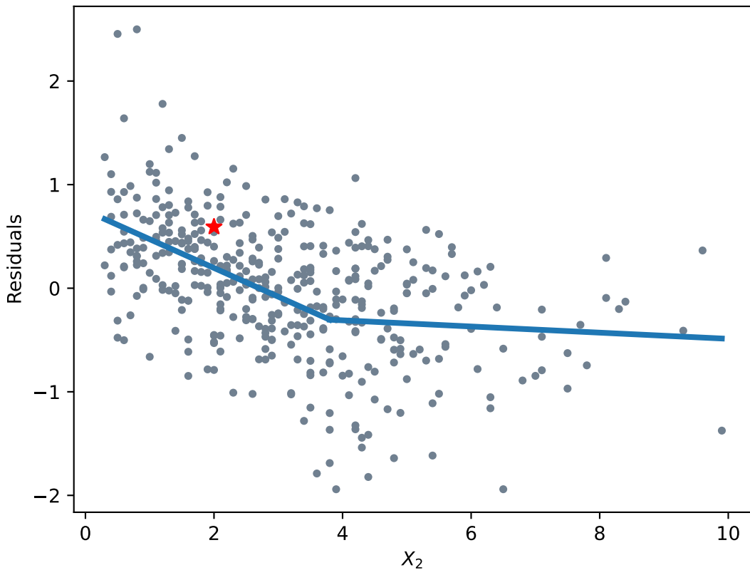
Depth = 2 - Node: BLIN - Feature: X_2 - Pivot: 3.8
