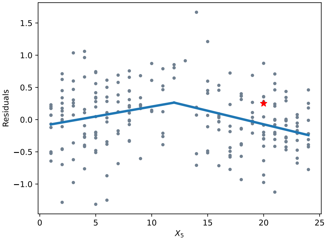
Depth = 5 - Node: BLIN - Feature: X_5 - Pivot: 12.0
