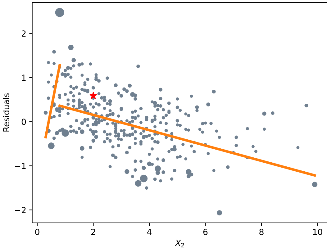
Depth = 2 - Node: PLIN - Feature: X_2 - Pivot: 0.8
