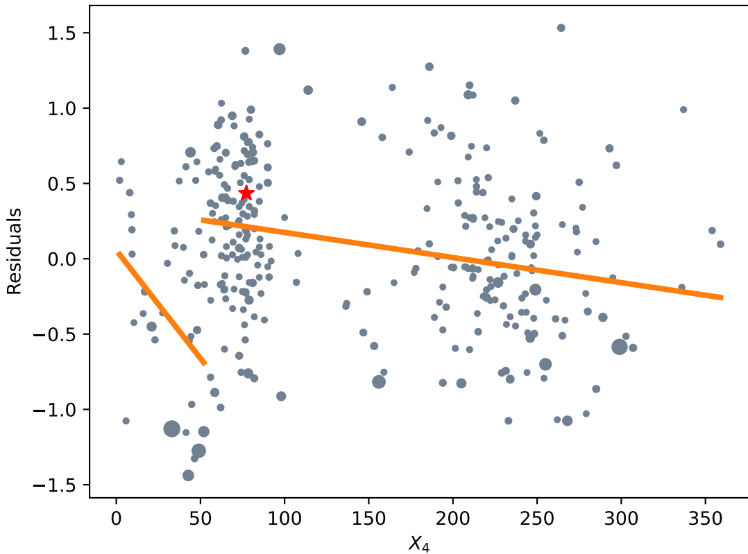
Depth = 3 - Node: PLIN - Feature: X_4 - Pivot: 52.0
