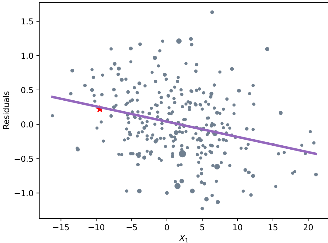
Depth = 4 - Node: LIN - Feature: X_1
