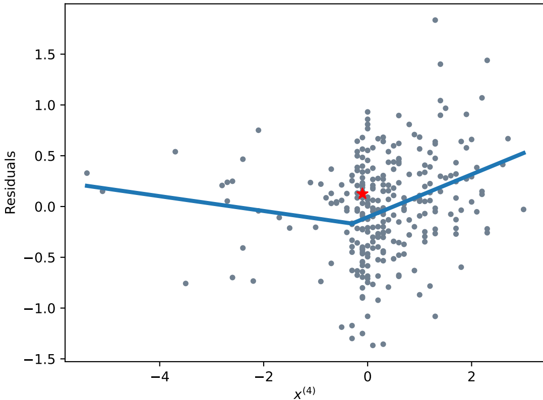
Depth = 4 - Node: BLIN - Feature: x^{(4)} - Pivot: -0.3
