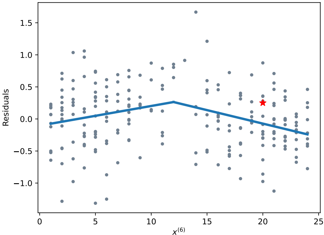
Depth = 5 - Node: BLIN - Feature: x^{(6)} - Pivot: 12.0
