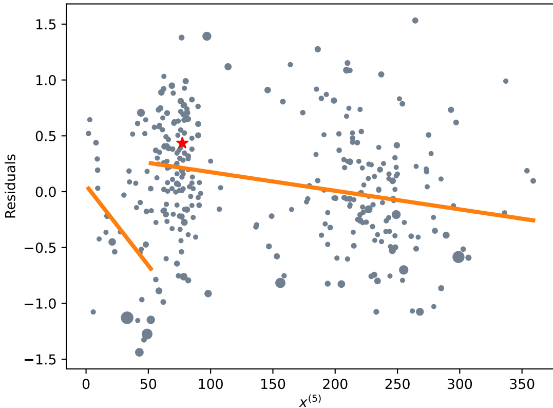
Depth = 3 - Node: PLIN - Feature: x^{(5)} - Pivot: 52.0
