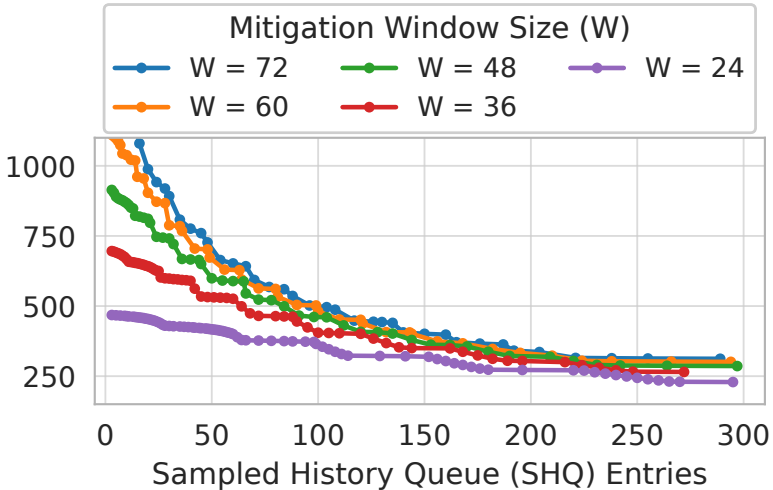
Double-Sided RowHammer Threshold ( T_{RH-D} )
