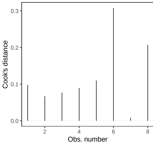
Cook's distance
