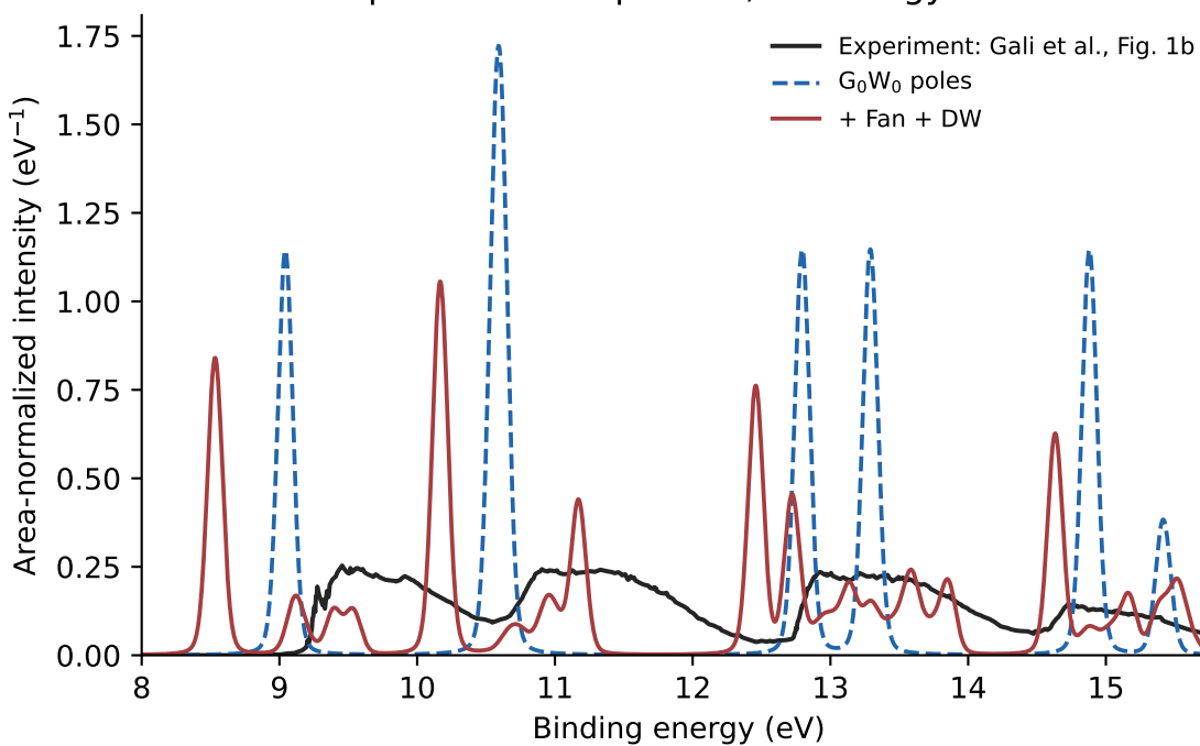
Experiment comparison; no energy shift
