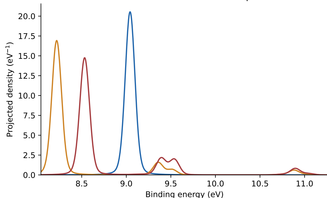
HOMO coupling; modes grouped within 1 \text{ cm}^{-1}
