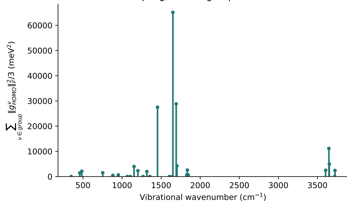
HOMO coupling; modes grouped within 1 \text{ cm}^{-1}
