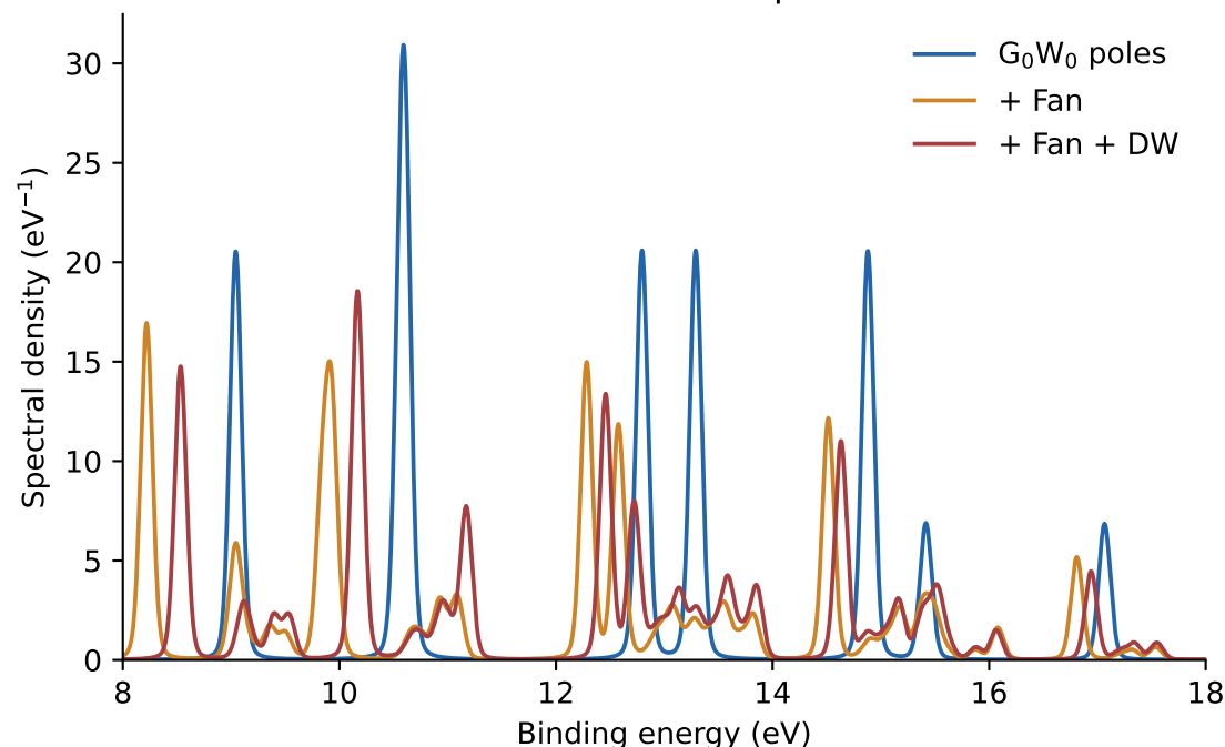
Experiment comparison; no energy shift
