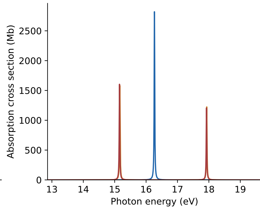
Native H2/3-21G, 300 K; frozen GW correction and BSE kernel First excitation and satellite
