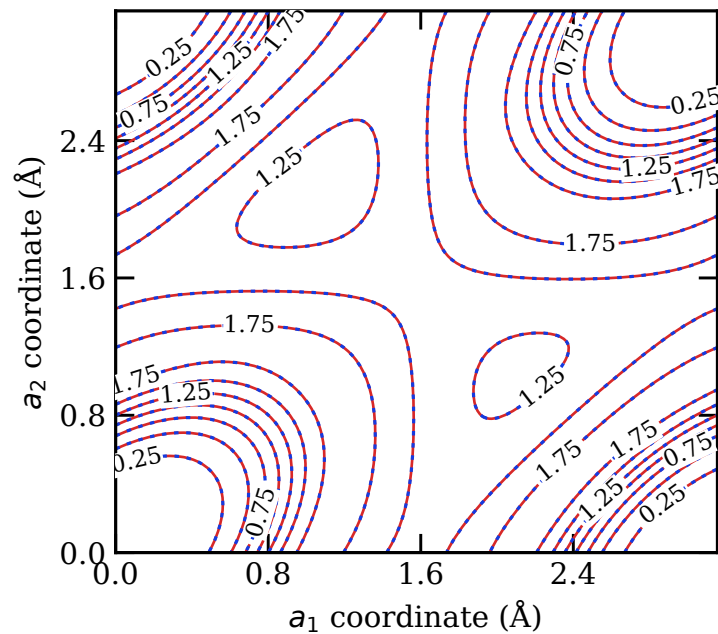
(c) Mg (0001)
