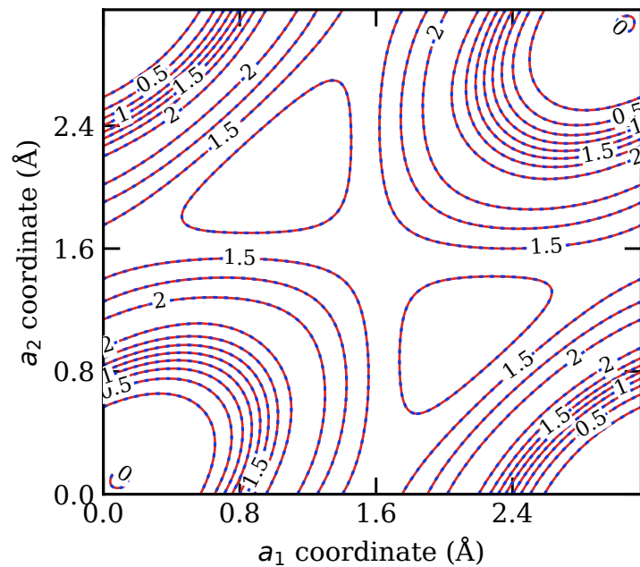
(c) Mg (0001)
