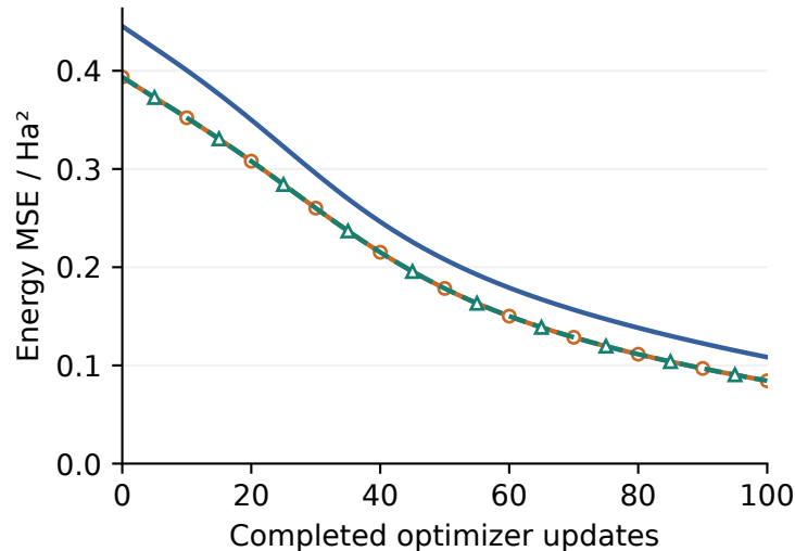
MSE component
