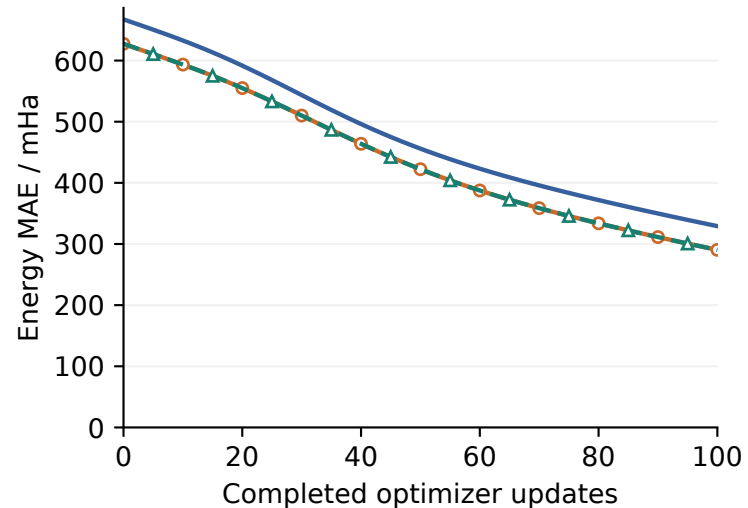
MAE component
