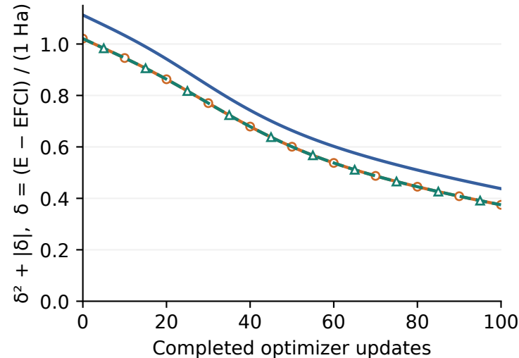
Total loss
