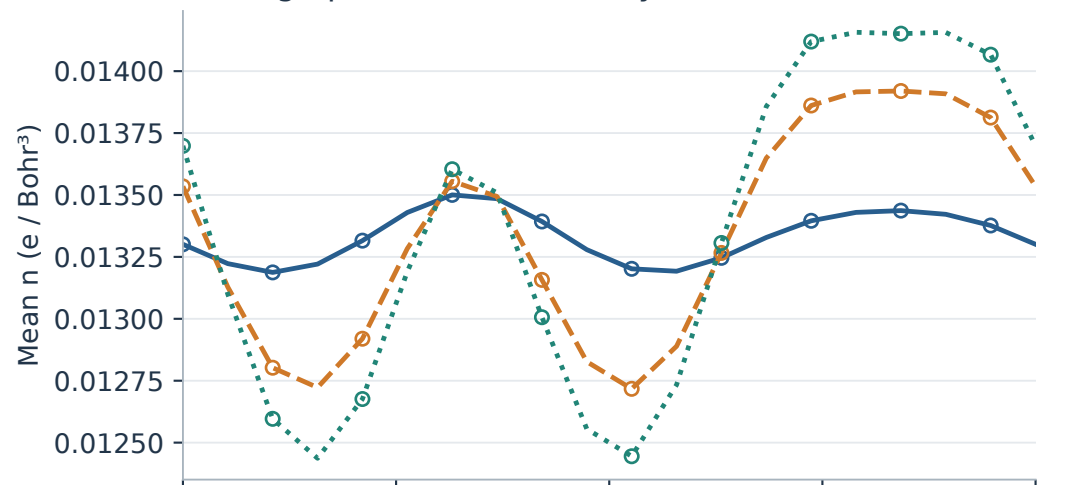
(b) Mg · planar mean density
