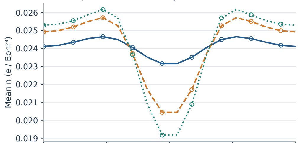
(a) Al · planar mean density
