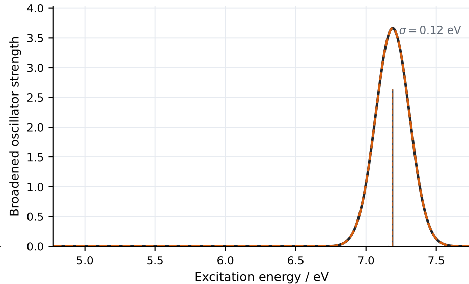
Benzene full TDDFT
