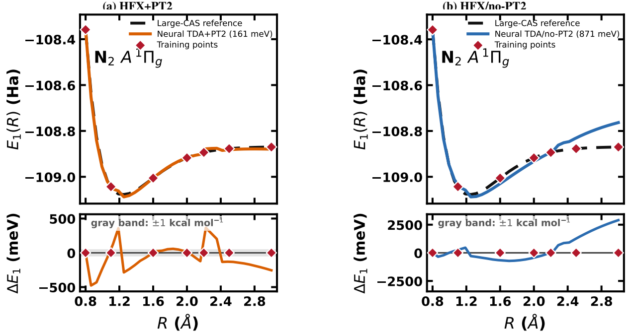
FIG. 6. \text{N}_2 A^1\Pi_g excited-state dissociation curves for neural TDA calculations with and without the PT2 channel. The plotted quantity is the total excited-state energy E_1(R) = E_0(R) + \Omega_1(R) , using the Hammami et al. large-CAS curve as the reference. 22 In each panel, the upper subpanel compares the learned curve with the reference values, while the lower subpanel shows the signed error \Delta E_1 = E_{1,\text{model}} - E_{1,\text{ref}} . Red diamonds denote the training geometries, and the gray band marks \pm 1 \text{ kcal mol}^{-1} . The PT2-channel model gives a dense-curve mean absolute error of 0.161 eV and a maximum absolute error of 0.477 eV, while removing the PT2 channel increases the corresponding errors to 0.871 eV and 2.905 eV.
