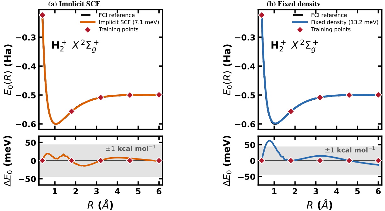
FIG. 3. H_2^+ X^2\Sigma_g^+ ground-state dissociation curves for the HFX-channel neural functional under implicit-SCF and fixed-density training. In each panel, the upper subpanel compares the learned curve with the one-electron FCI reference values, while the lower subpanel shows the signed error \Delta E_0 = E_{0,\text{model}} - E_{0,\text{ref}} . Red diamonds denote the five training geometries, and the gray band marks \pm 1 \text{ kcal mol}^{-1} . The implicit-SCF model gives a dense-curve mean absolute error of 7.1 meV and a maximum absolute error of 19.2 meV. Fixed-density training gives corresponding errors of 13.2 meV and 63.2 meV.
