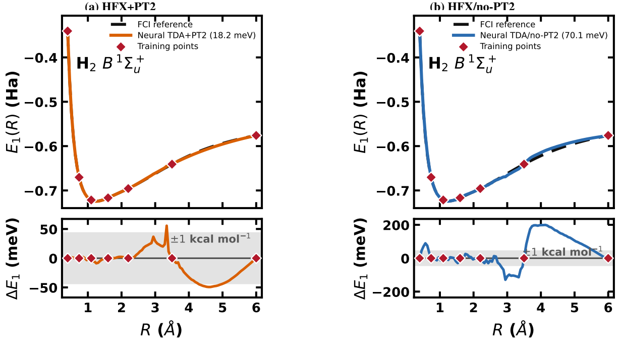
FIG. 5. \text{H}_2 B^1\Sigma_u^+ excited-state dissociation curve for neural TDA calculations with and without the PT2 channel. The plotted quantity is the total excited-state energy E_1(R) = E_0(R) + \Omega_1(R) . In each panel, the upper subpanel compares the learned curve with the FCI reference values, while the lower subpanel shows the signed error \Delta E_1 = E_{1,\text{model}} - E_{1,\text{ref}} . Red diamonds denote the training geometries, and the gray band marks \pm 1 \text{ kcal mol}^{-1} . The PT2-channel model gives a dense-curve mean absolute error of 18.2 meV and a maximum absolute error of 55.6 meV, whereas the updated no-PT2 model gives corresponding errors of 70.1 meV and 199.3 meV.
