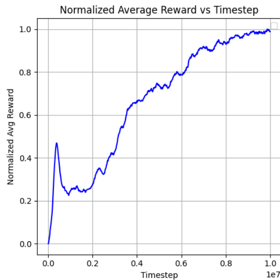
Figure 5.6: Training curves for Pursuit - Sum Aggregation
