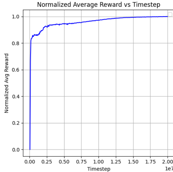
Figure 5.4: Training curves for Simple Spread - Sum Aggregation
