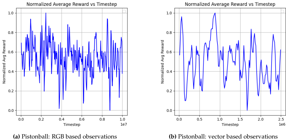
Figure 5.2: Training curves for Pistonball - Sum Aggregation
