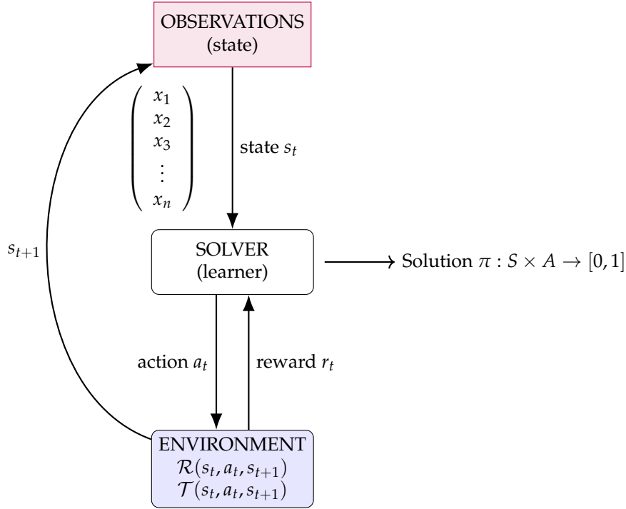
Figure 2.1: Agent-environment interaction loop in Reinforcement Learning
