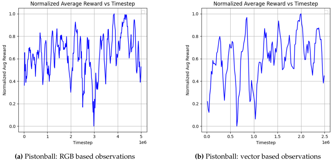
Figure 5.3: Training curves for Pistonball with Discrete action space - Sum Aggregation
