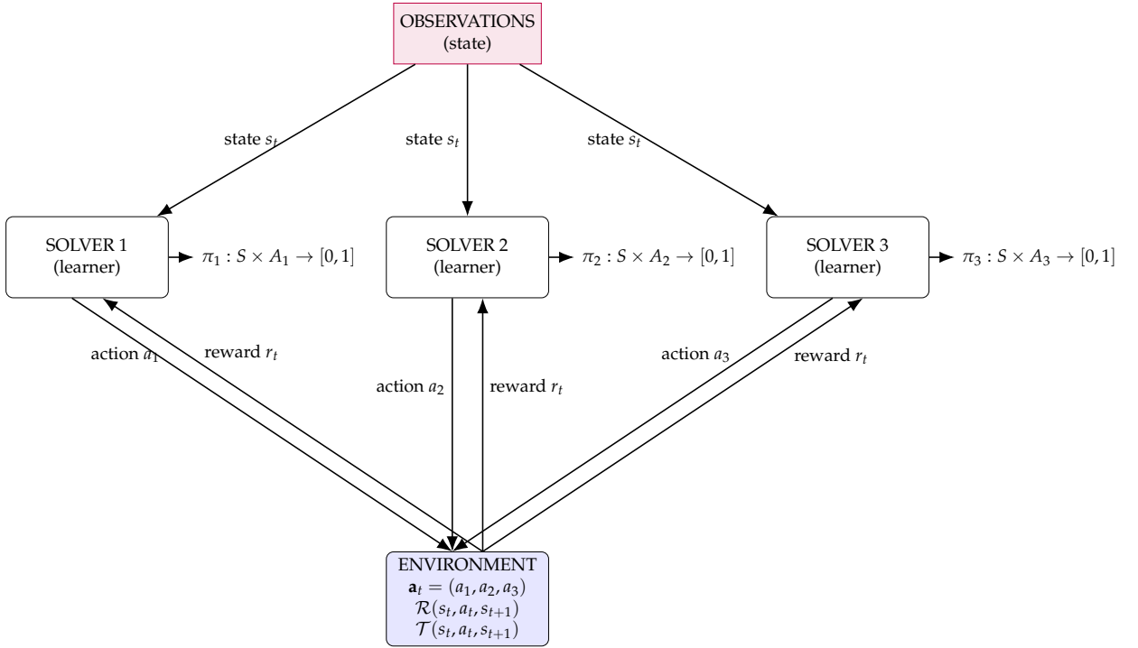
Figure 2.2: Agents-environment interaction loop for MMDPs
