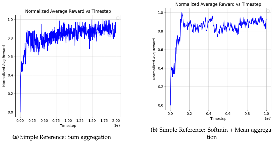
Figure 5.9: Training curves for Simple Reference
