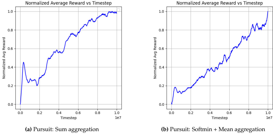
Figure 5.10: Training curves for Cooperative Pursuit
