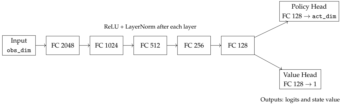
Figure 4.1: Neural network architecture used for PPO: shared MLP encoder with policy and value heads.
