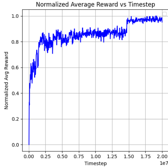
Figure 5.5: Training curves for Simple Speaker Listener - Sum Aggregation
