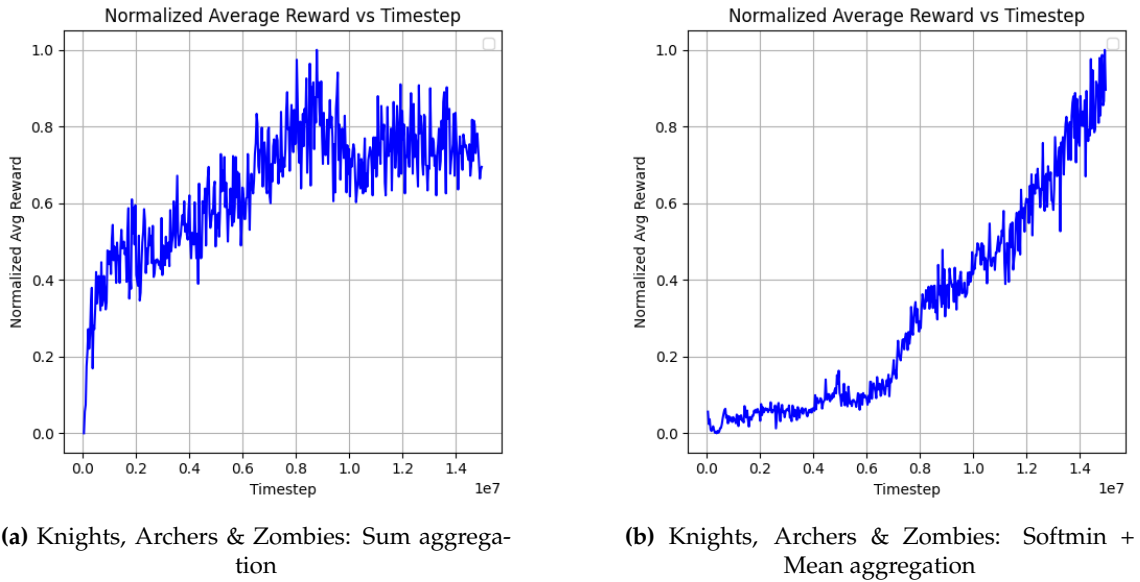
Figure 5.8: Training curves for Knights, Archers & Zombies
