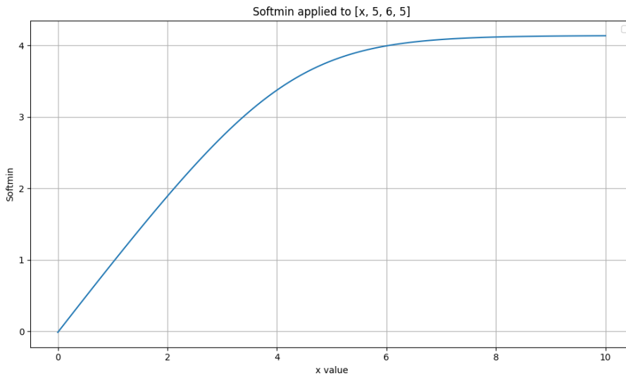
Figure 3.3: Softmin behaviour for reward vector (x, 5, 6, 5)
