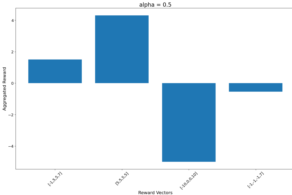
Figure 3.4: SoftminMean behaviour for different reward vectors
