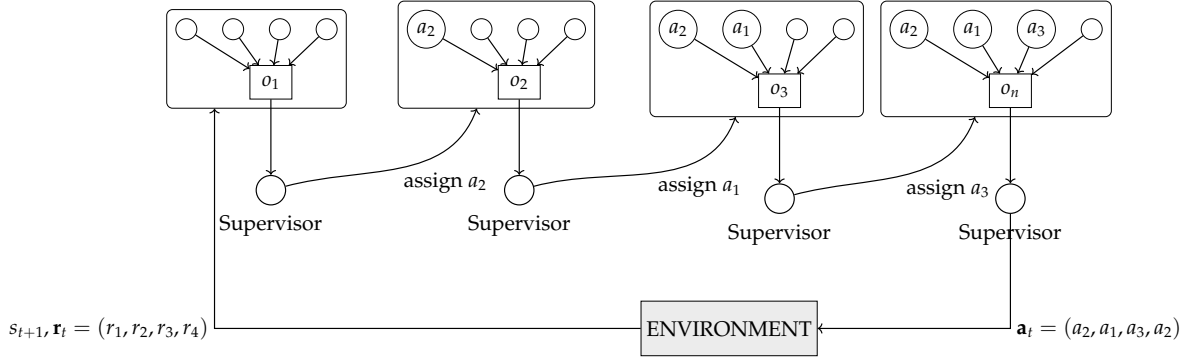
Figure 3.2: Joint action construction using supervisor meta-agent.
