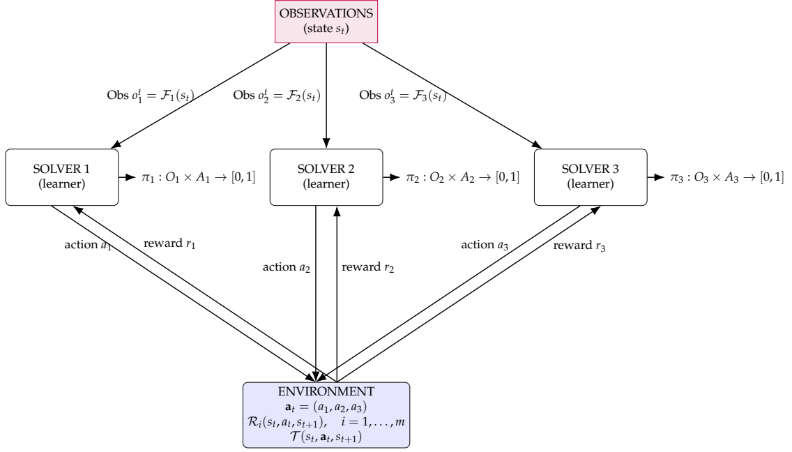
Figure 3.1: Agent-environment interaction loop for GMARL
