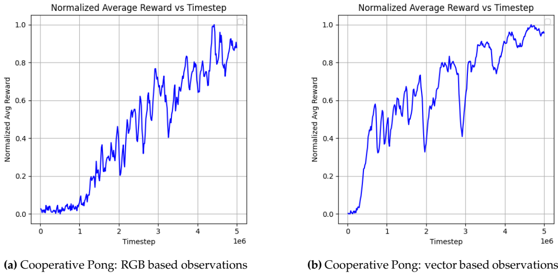
Figure 5.1: Training curves for Cooperative Pong - Sum Aggregation
