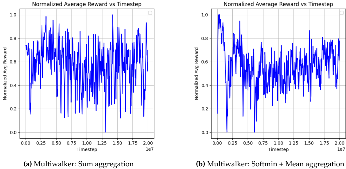
Figure 5.11: Training curves for Cooperative Multiwalker
