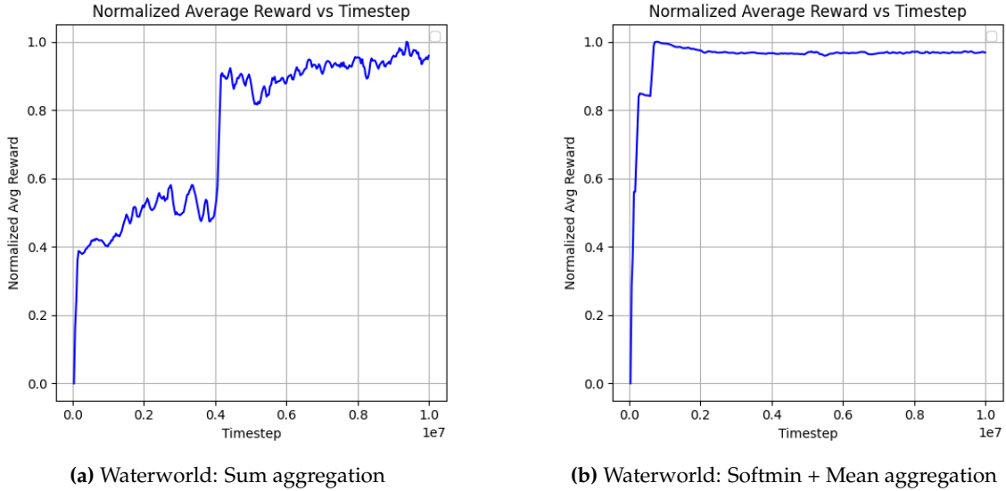
Figure 5.12: Training curves for Waterworld
