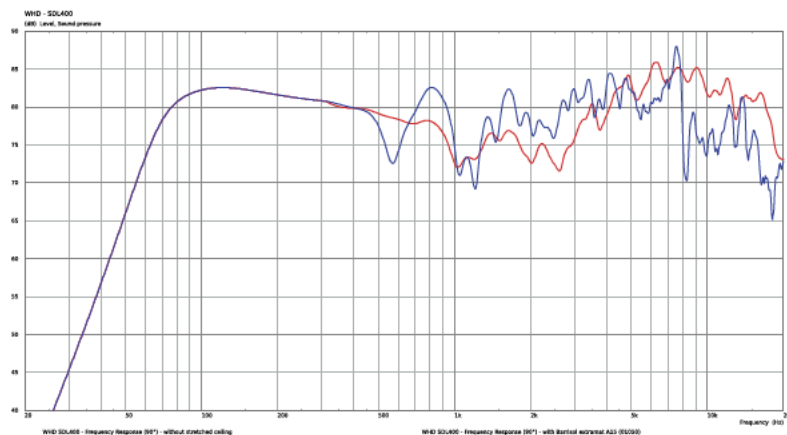
Loudspeaker without stretch ceiling Loudspeaker with stretch ceiling
