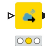
GET Request
