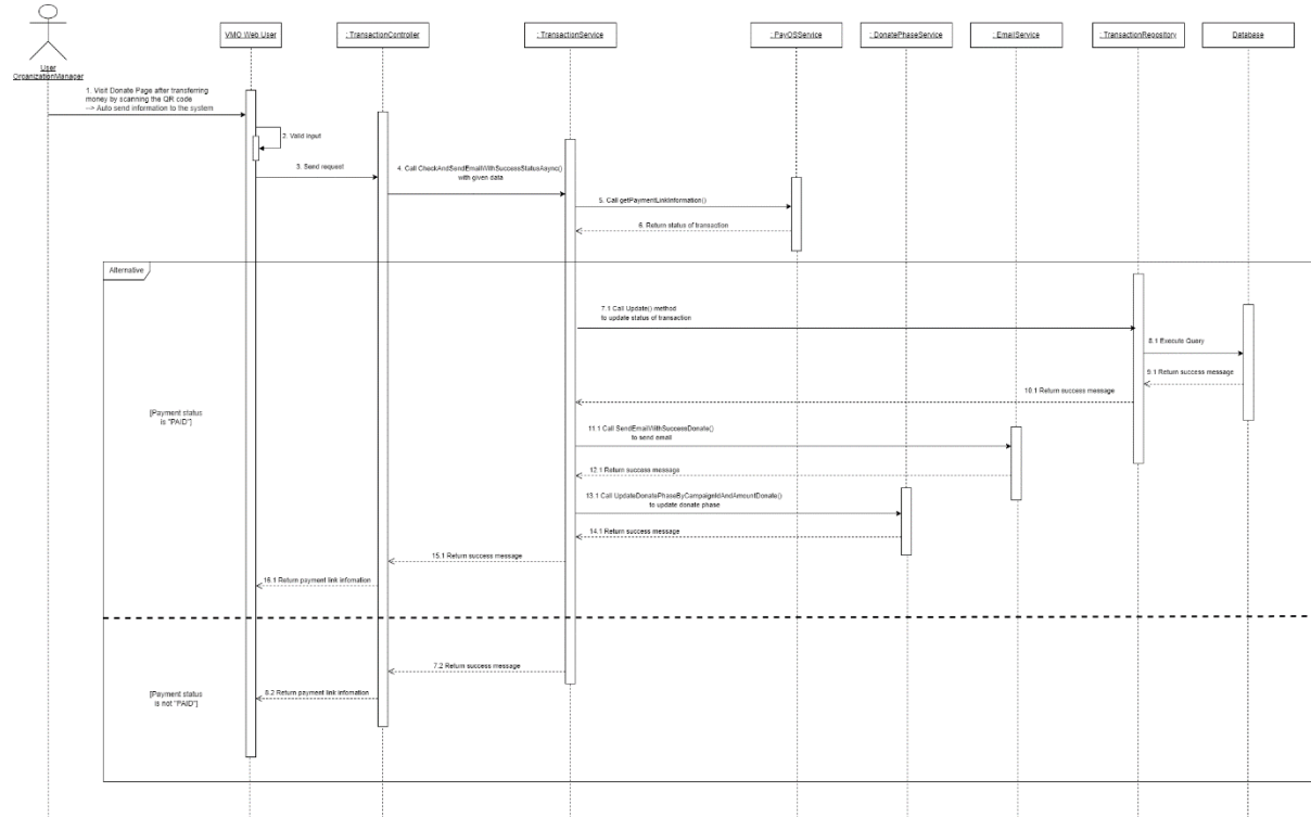
Figure 124 - Sequence Diagram - After Donate Money
