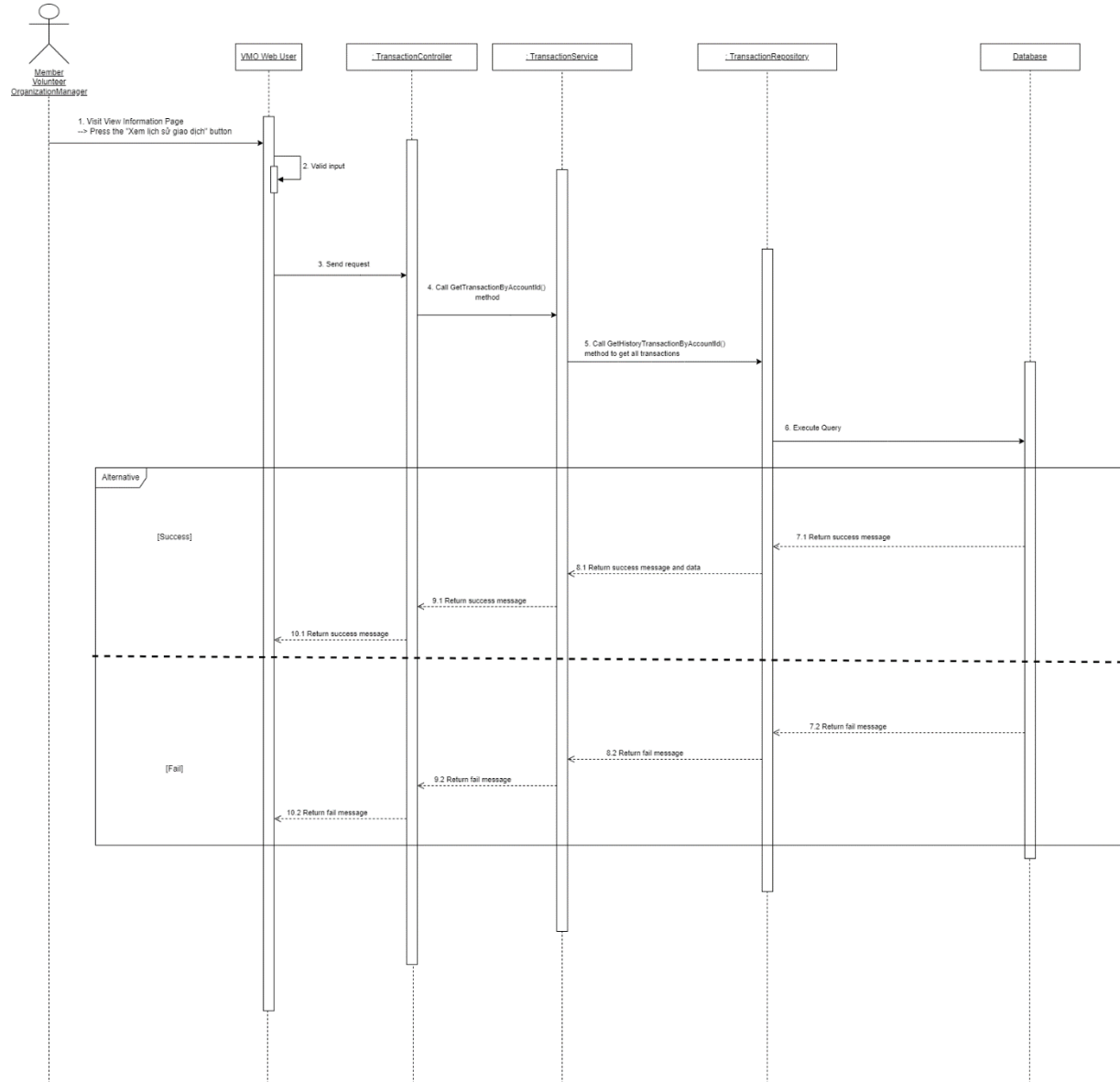
Figure 127 - Sequence Diagram - View History
