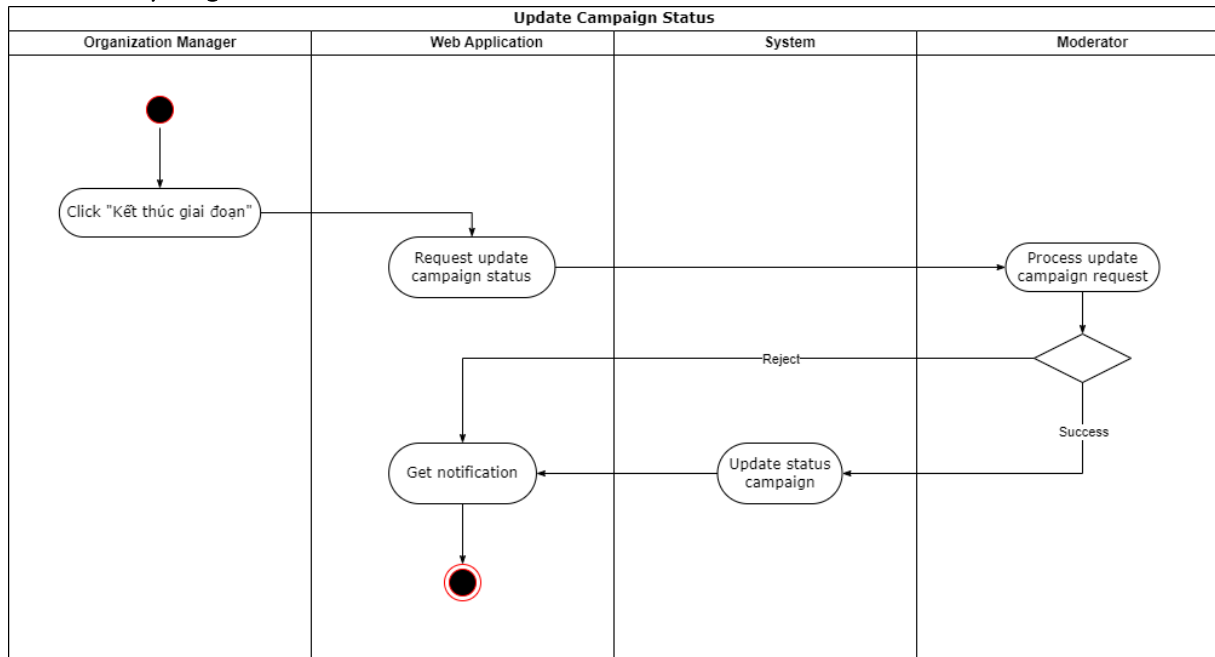
Figure 134 - Activity Diagram - Update Campaign Status
