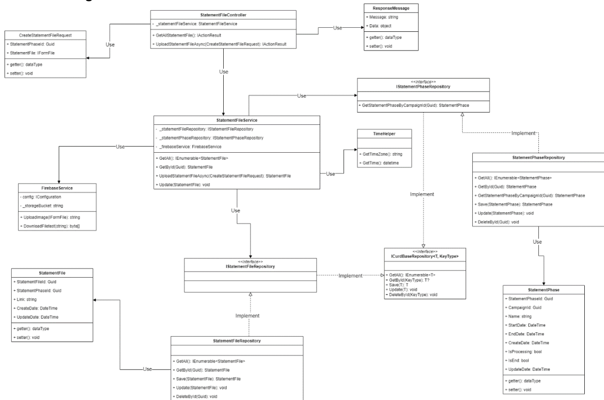
Figure 138 - Class Diagram - Upload Donation Document
