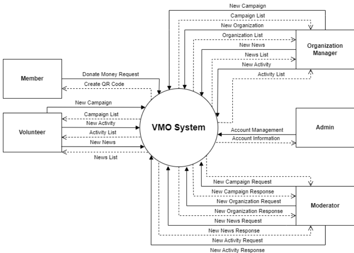
Figure 2 - Context Diagram
