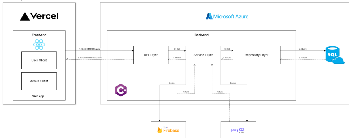
Figure 118 - System Architecture
