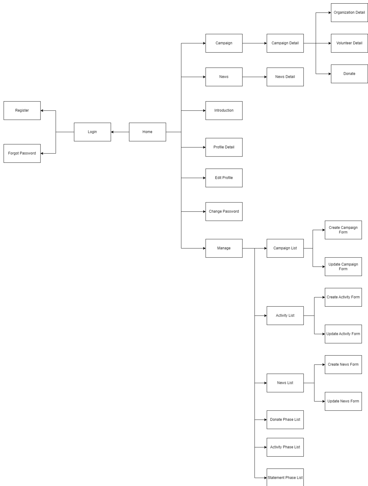
Figure 6 - Screen Flow - Volunteer
