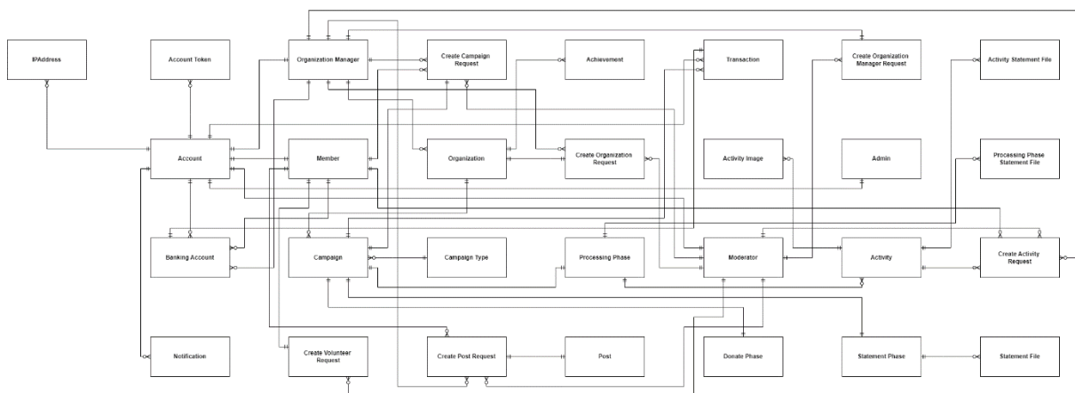
Figure 10 - Conceptual Diagram
