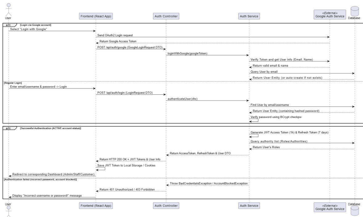
Figure 15: System Login Regular and Google OAuth Sequence Diagram
