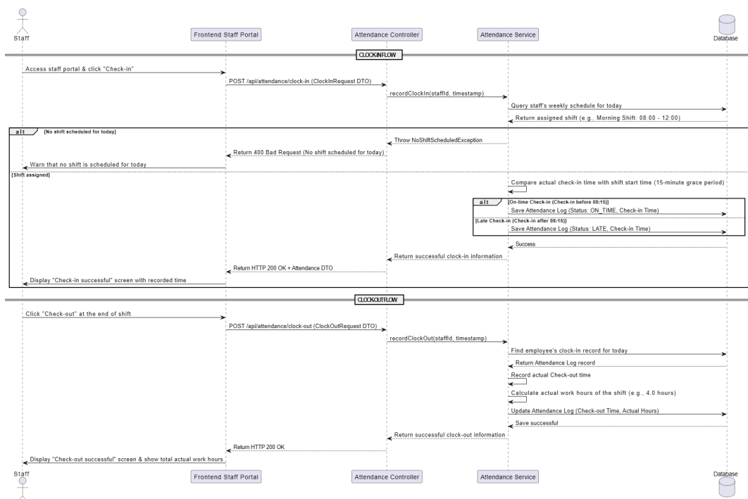
Figure 21: Staff Check-in and Check-out Attendance Sequence Diagram
