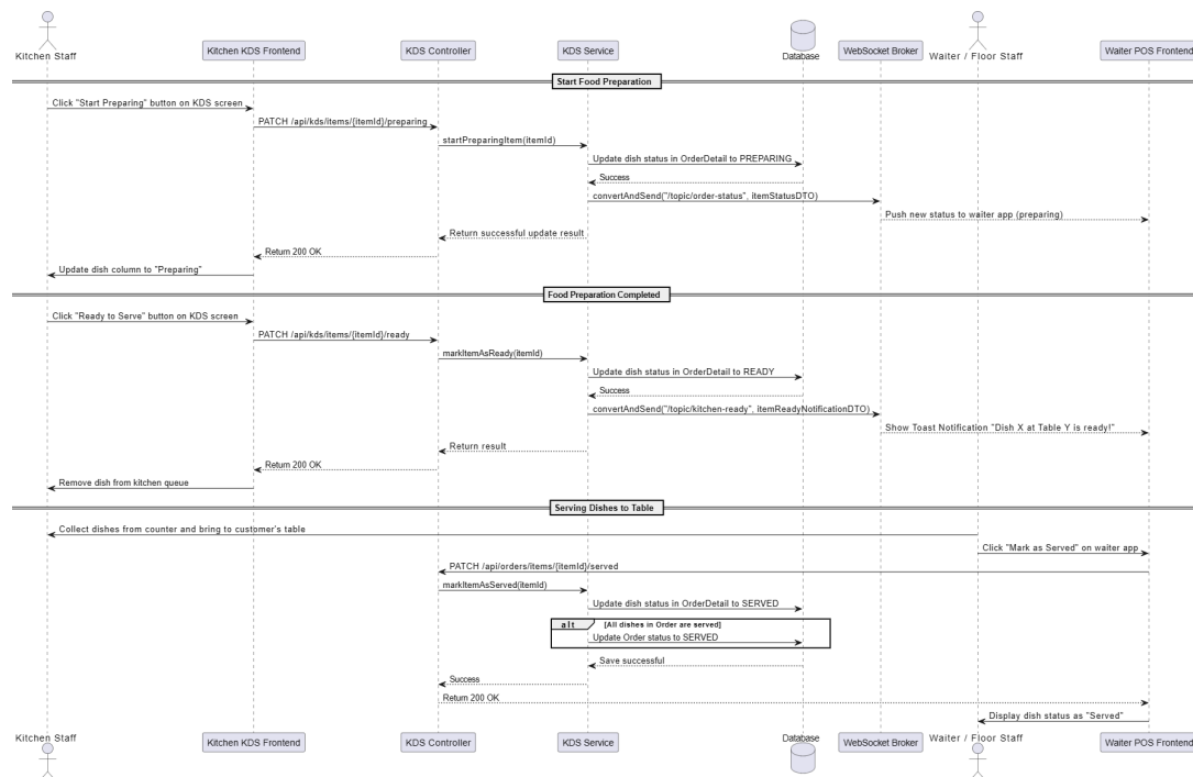
Figure 19: Kitchen Cooking Process and WebSocket Status Synchronization Sequence Diagram
