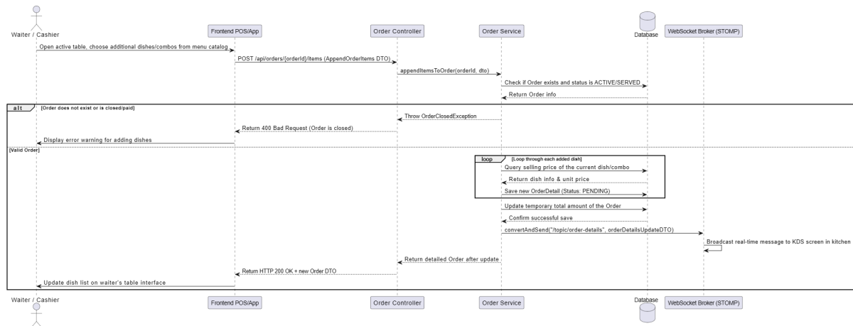
Figure 18: Add Dishes and Combos at Dine-in Table Sequence Diagram
