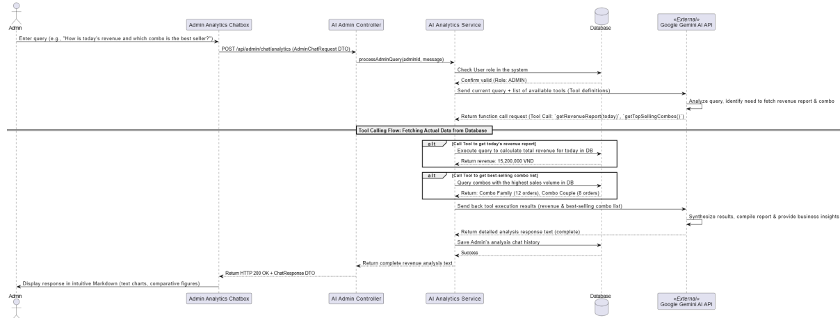
Figure 23: Admin Real-time Revenue Query via Gemini AI Tool Calling Sequence Diagram
