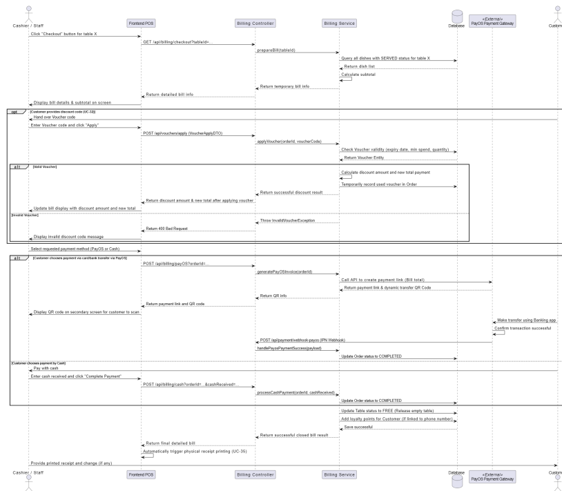
Figure 20: Counter Bill Payment, Voucher Application, and Bill Printing Sequence Diagram
