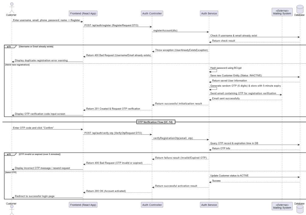
Figure 14: Customer Account Registration and Email OTP Verification Sequence Diagram
