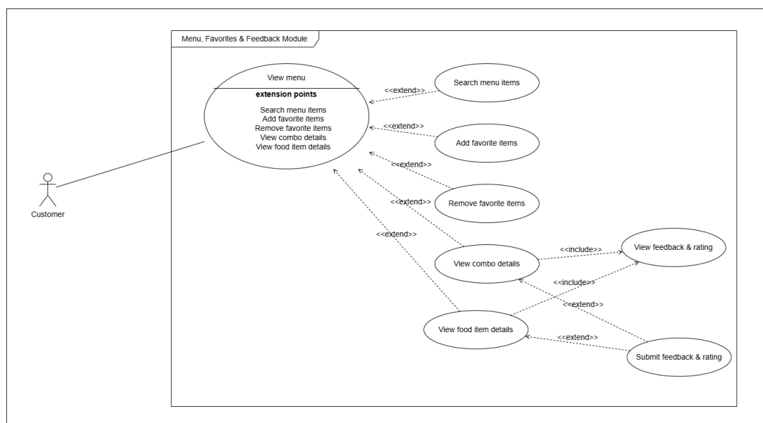
Figure I-5: Detailed Use Case Diagram for Viewing Menu, Favorites and Feedback
