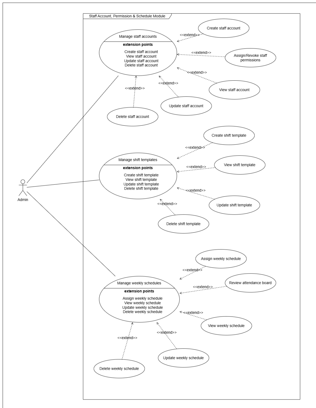
Figure I-11: Detailed Use Case Diagram for Staff Account, Permission and Schedule Management
