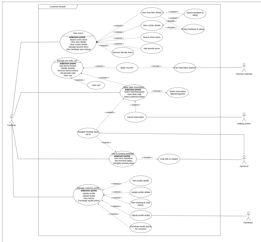
Figure I-2: Overview Use Case Diagram for Customer Site
