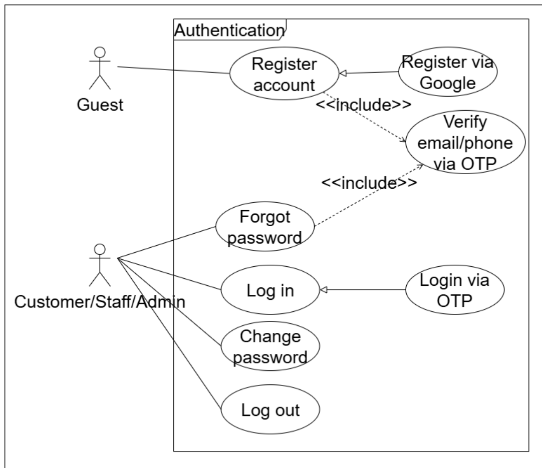
Figure I-1: Overview Use Case Diagram for Authentication
