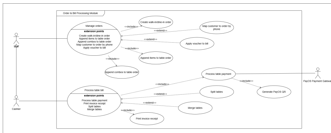
Figure I-7: Detailed Use Case Diagram for Order and Bill Processing
