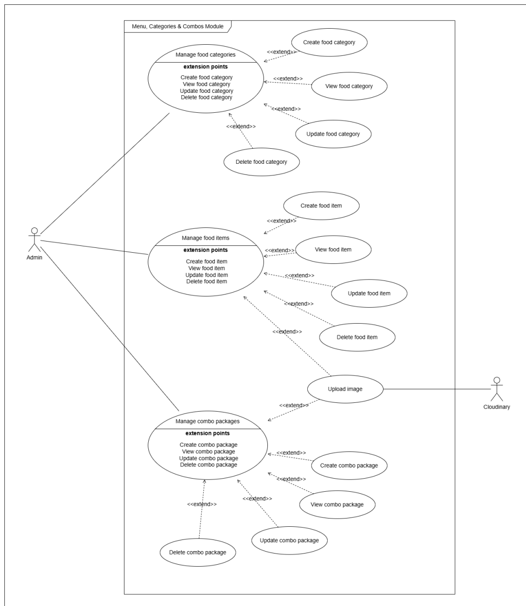
Figure I-10: Detailed Use Case Diagram for Managing Menu, Categories and Combos
