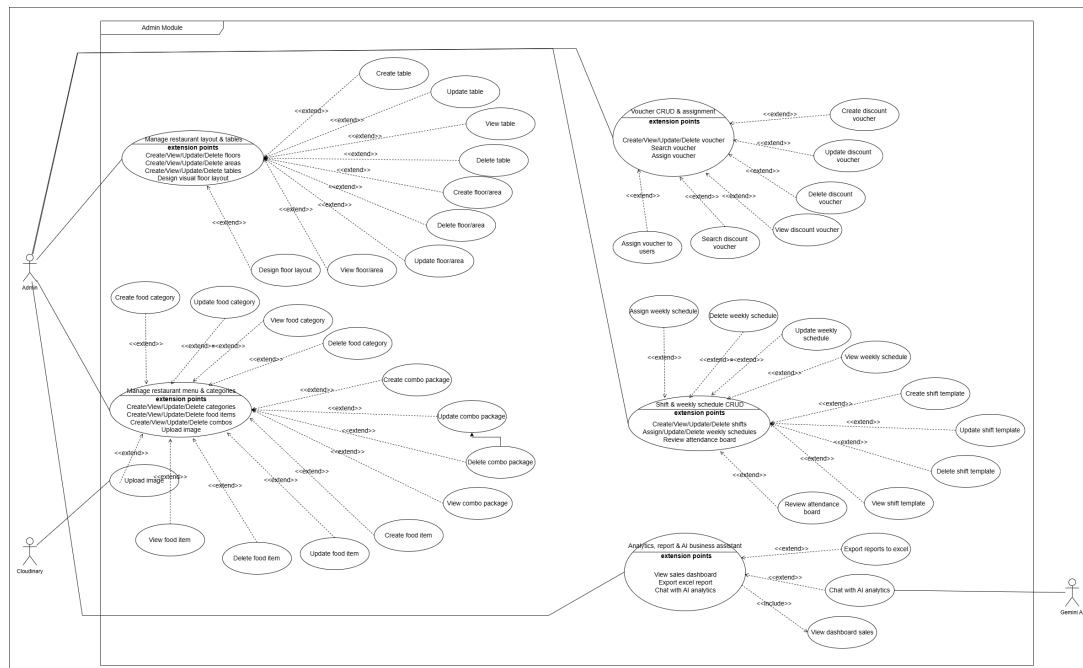
Figure I-4: Overview Use Case Diagram for Administration Site
