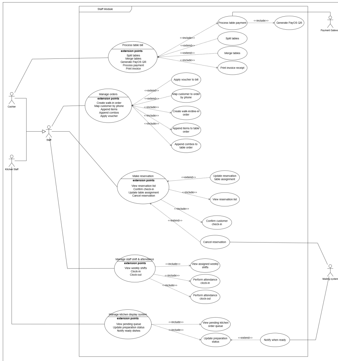
Figure I-3: Overview Use Case Diagram for Staff Site
