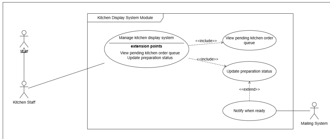
Figure I-8: Detailed Use Case Diagram for KDS and Order Preparation
