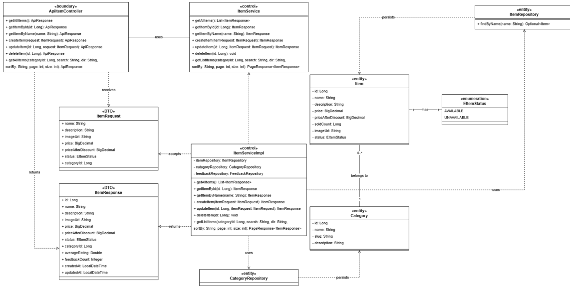
Figure III-8: Detailed Design Class Diagram for Manage Item Use Case
