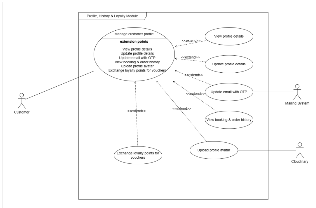
Figure I-6: Detailed Use Case Diagram for Managing Profile, History and Loyalty
