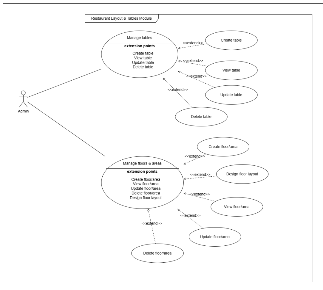
Figure I-9: Detailed Use Case Diagram for Managing Restaurant Layout and Tables
