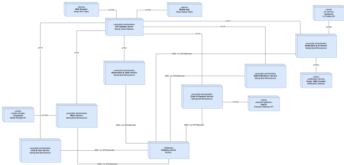
Figure V-1: Deployment Diagram for the CrownDine System Architecture Based on Service-Oriented Architecture
