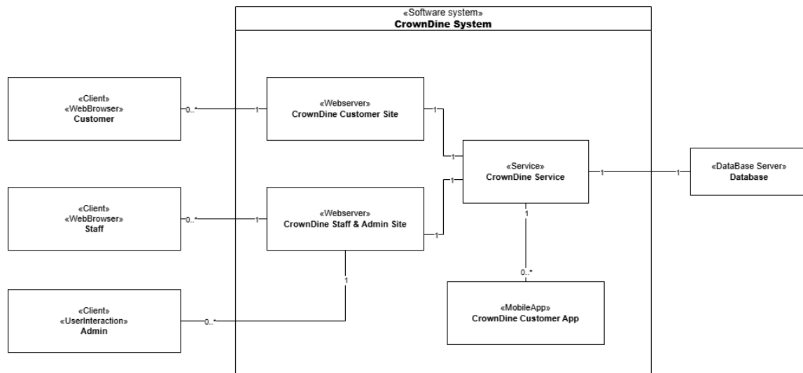
Figure V-2: Class Diagram for the System Architecture Based on Service-Oriented Architecture
