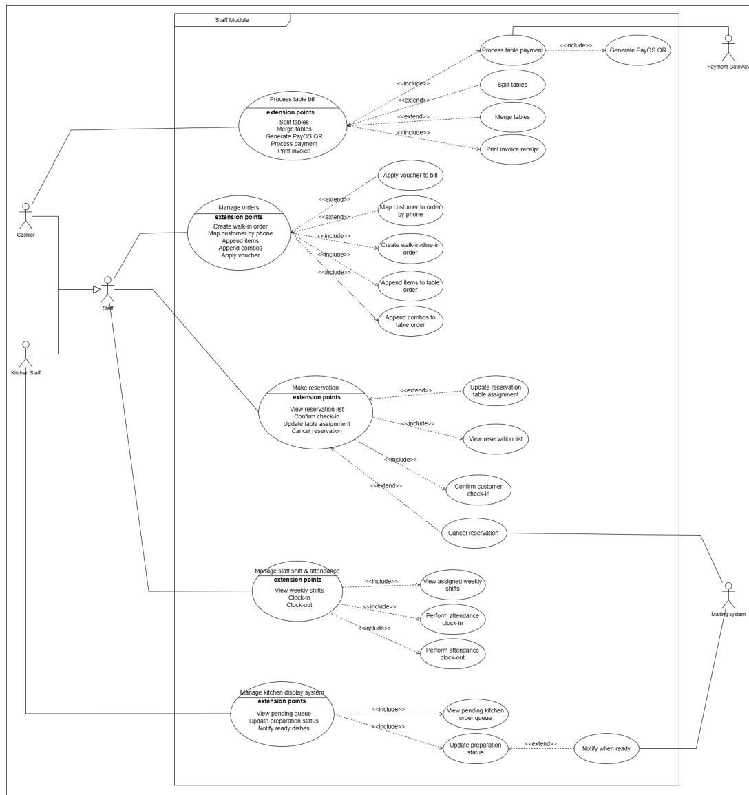
Figure I-3: Overview Use Case Diagram for Staff Site
