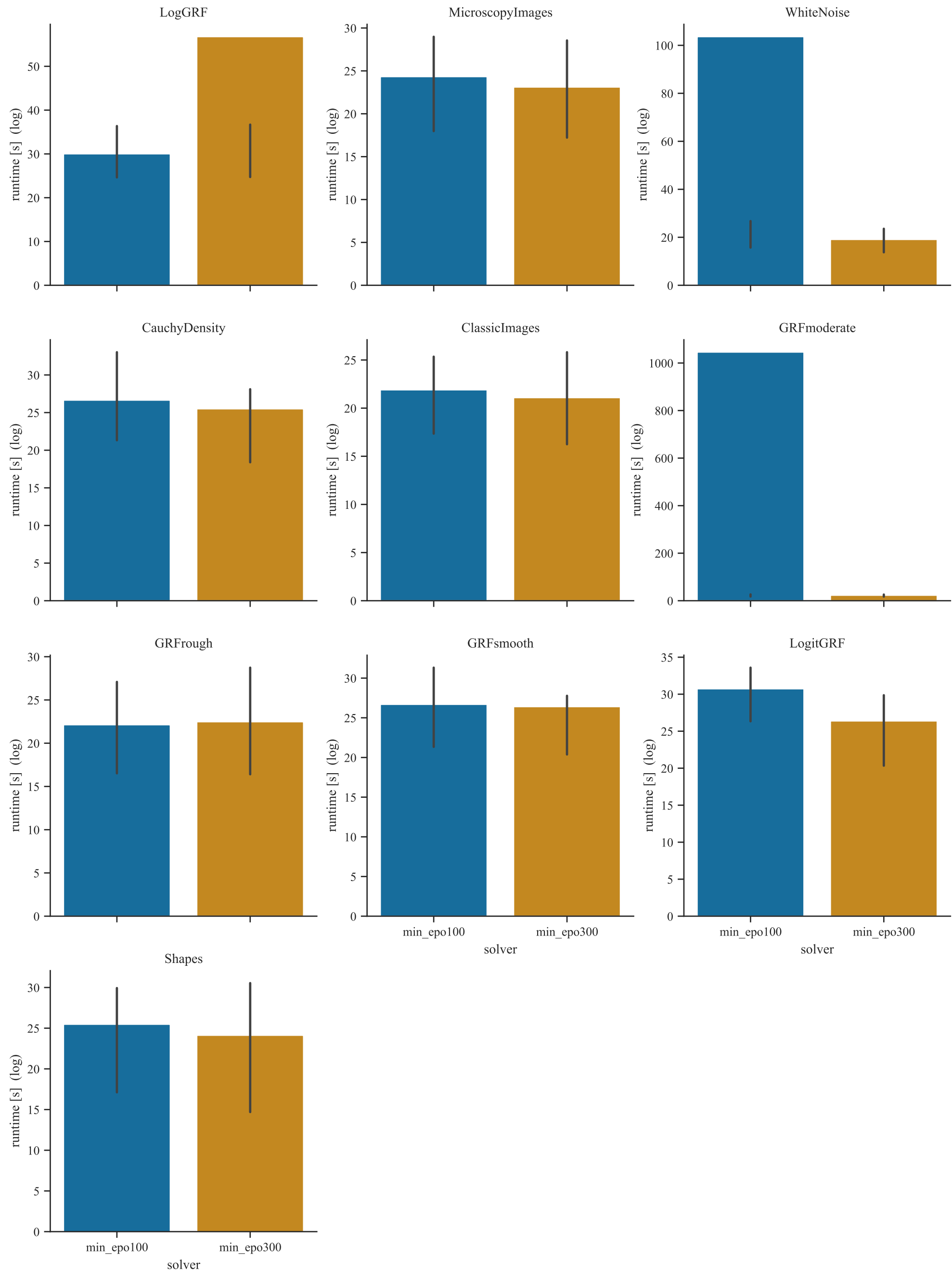
Runtime per solver, per DOTmark class
